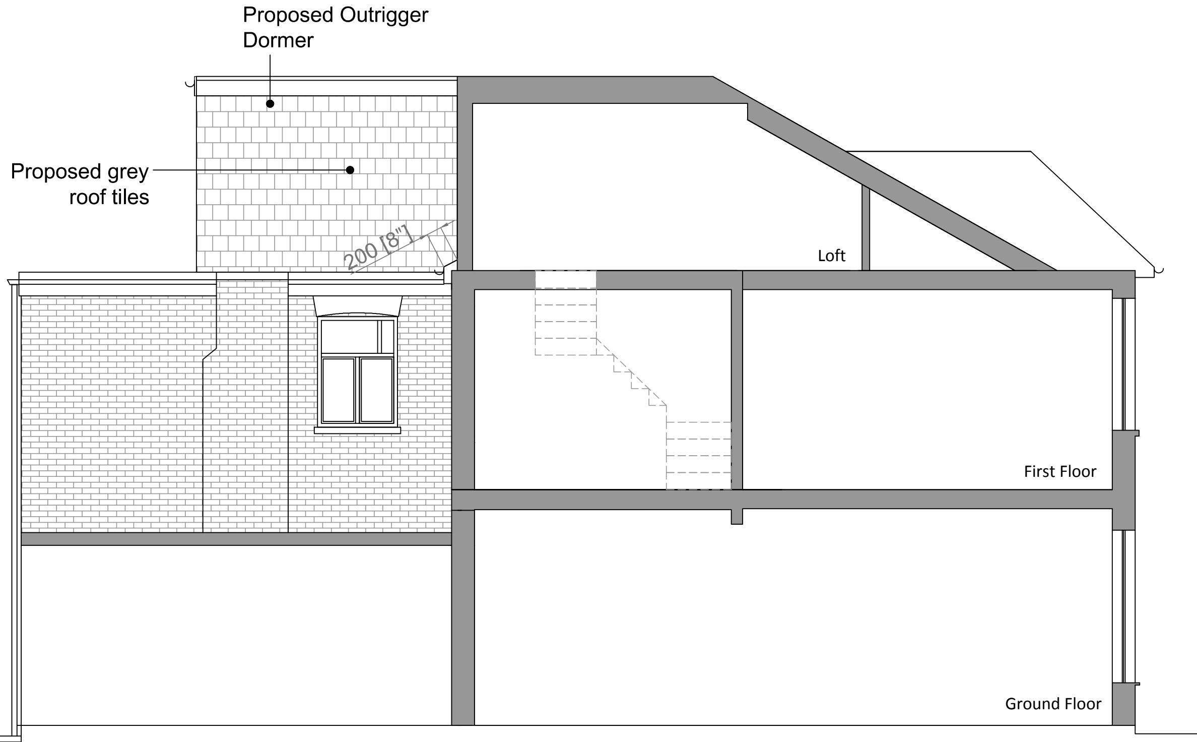
Proposed Section/Side Elevation
