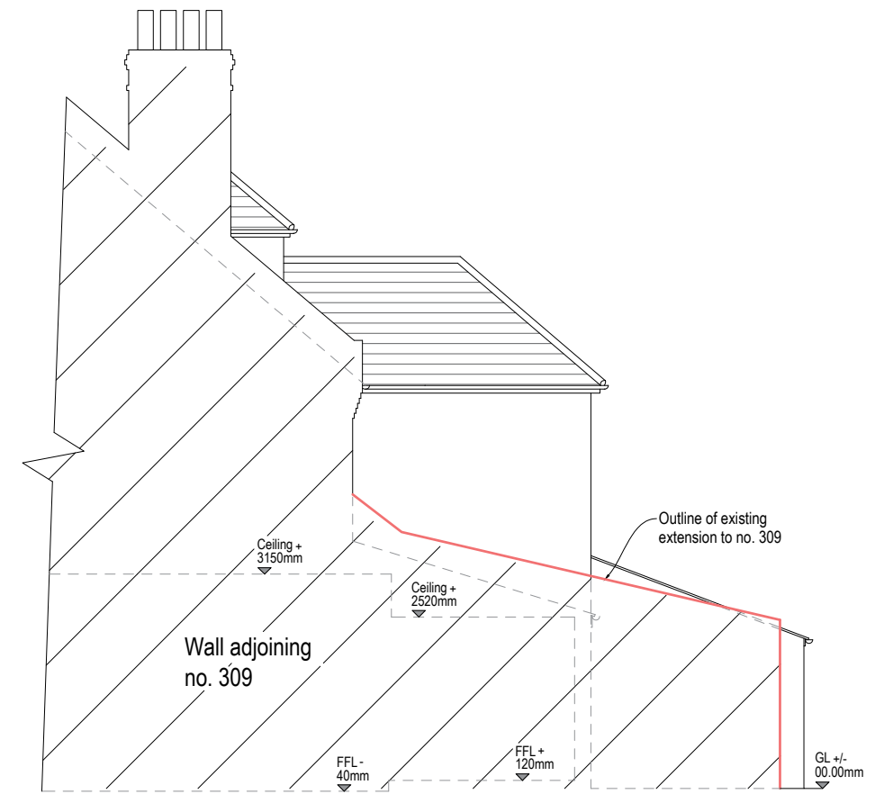
Side (SW) Elevation/Section Existing
