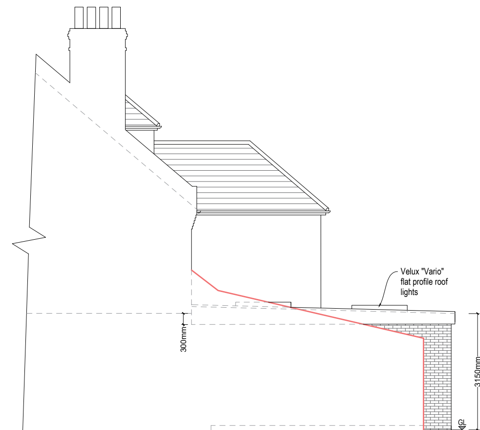
Side (SW) Elevation/Section Proposed
