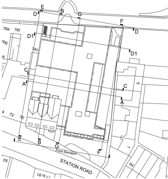
Key Plan 1:1000
