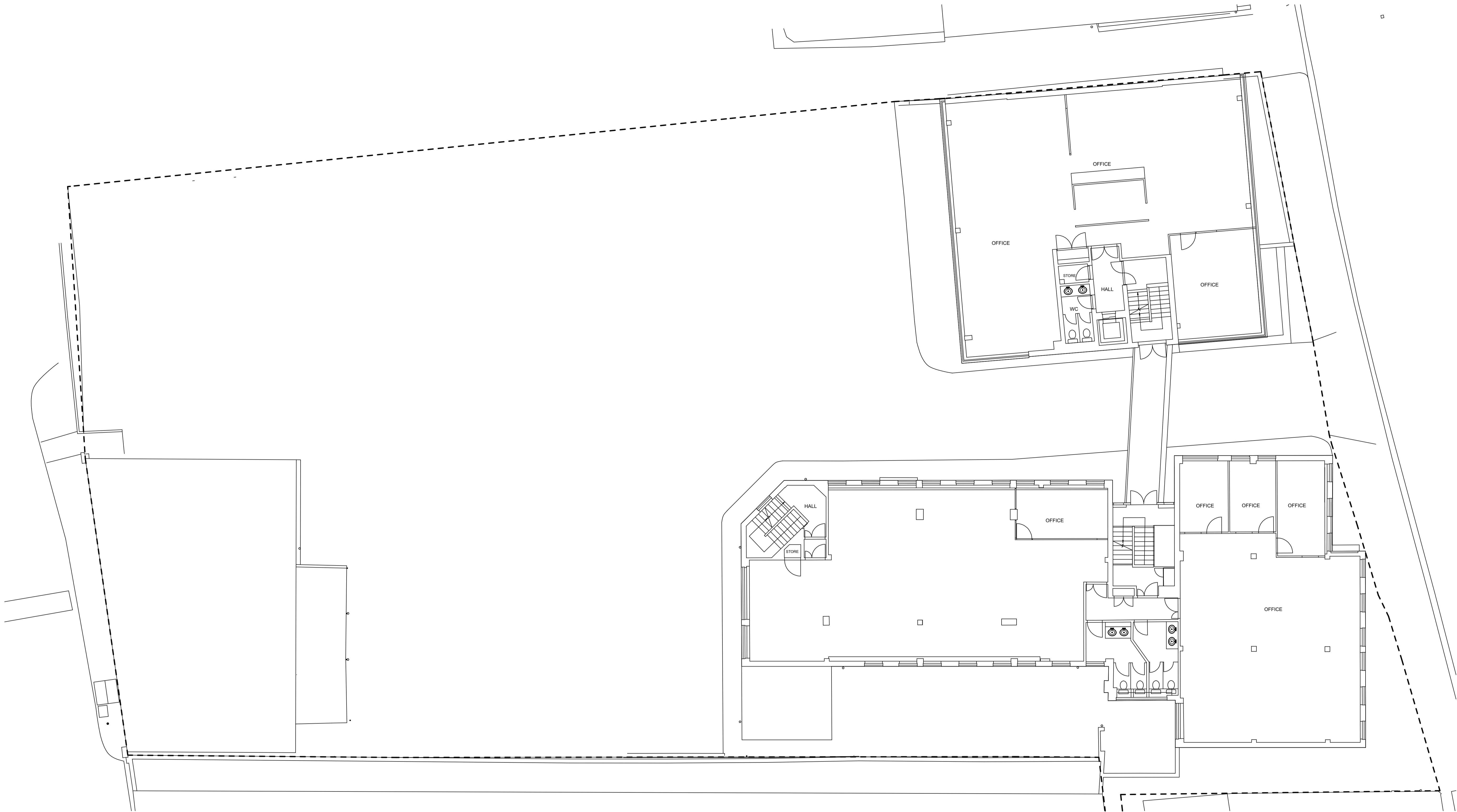
EXISTING - FIRST FLOOR PLAN
