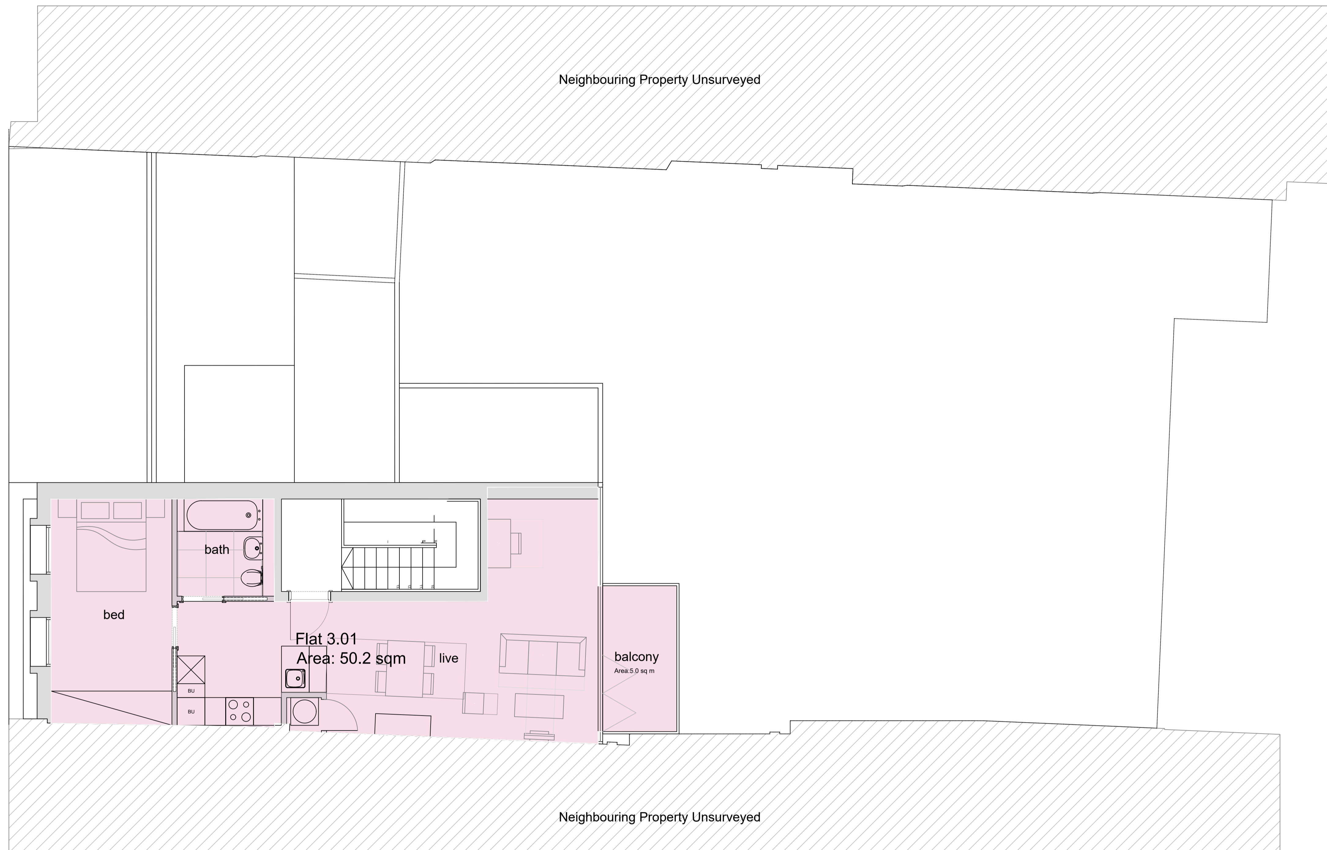
Third Floor Plan Scale: 1/50
