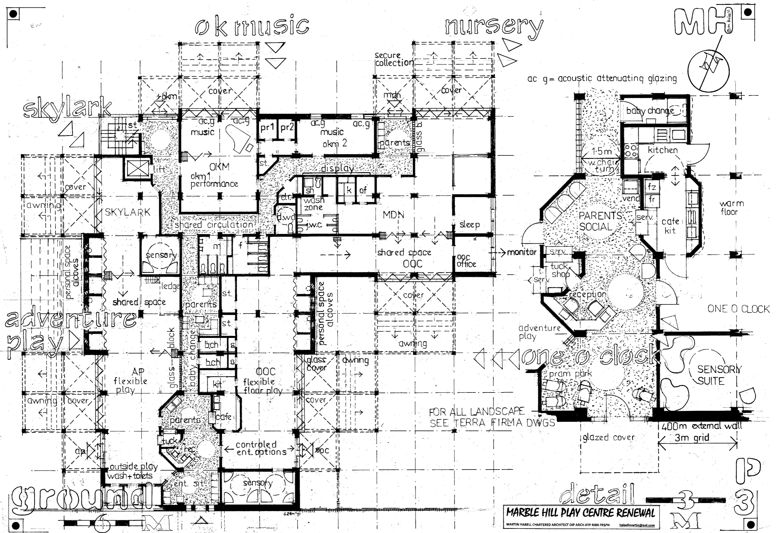
Figure 1 - Architectural proposals
