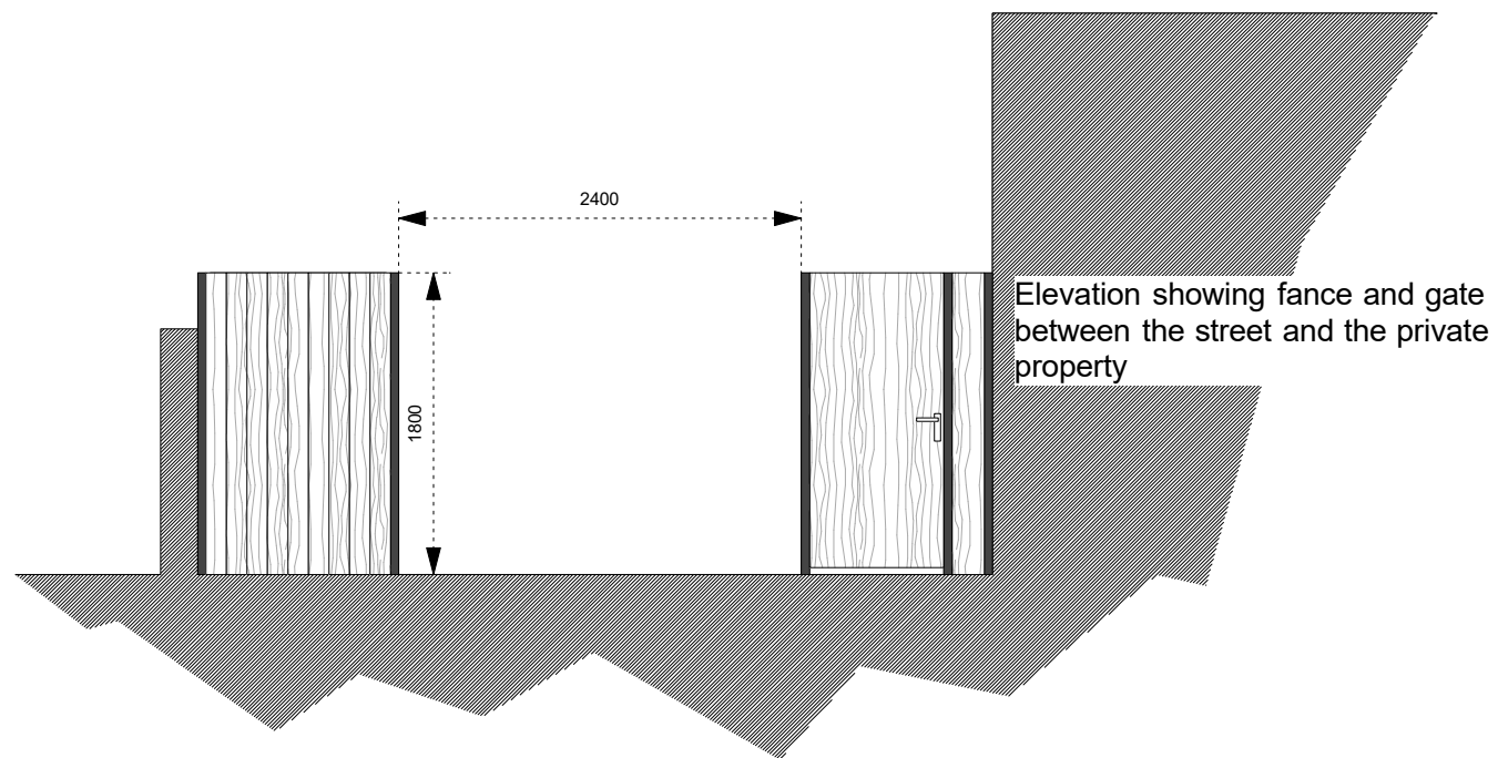
Front Elevation - Opened Gate
