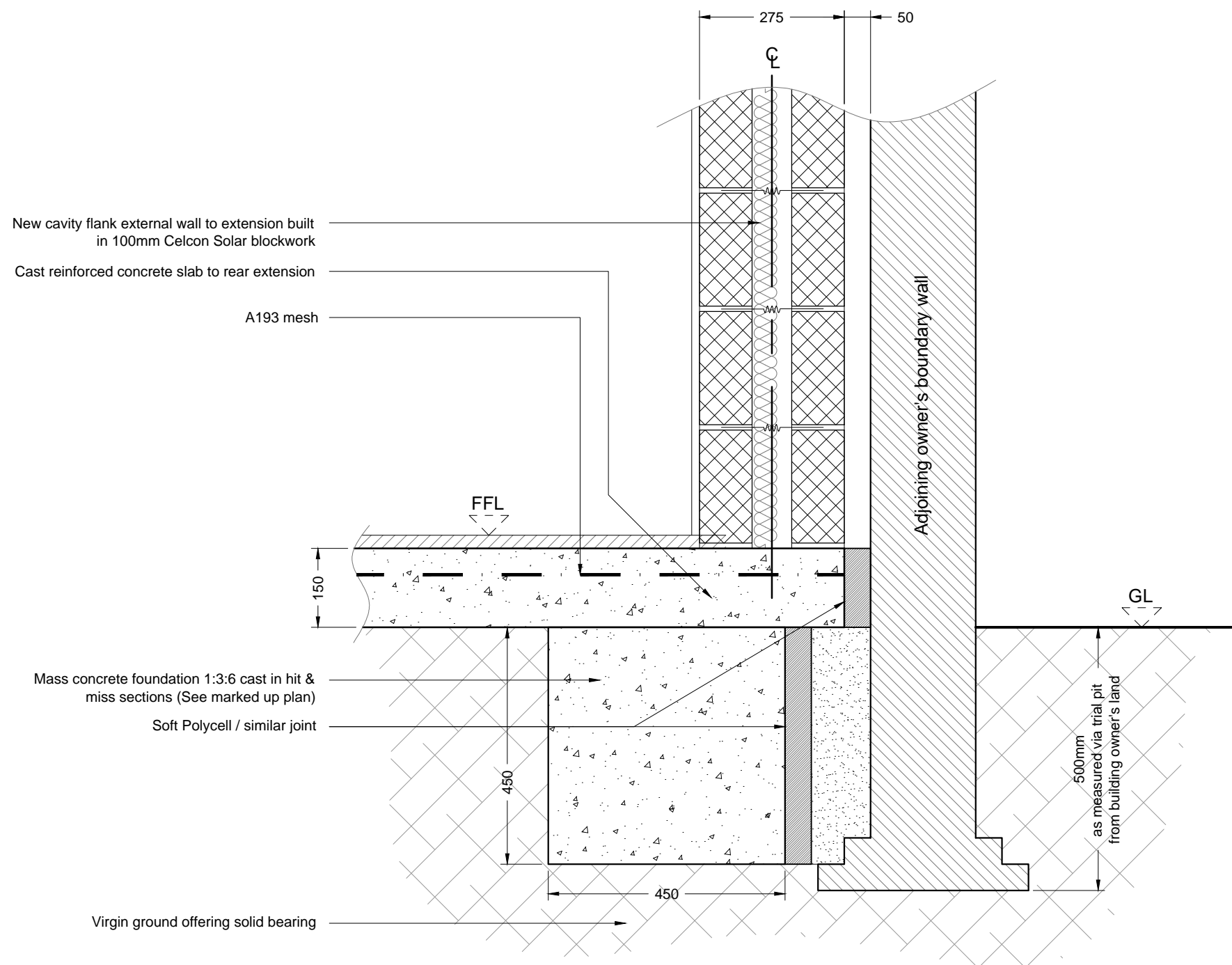
Proposed cross section detail of foundation to flank wall of extension
