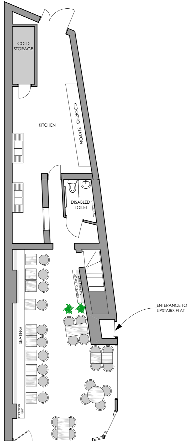
PROPOSED GROUND FLOOR 1:100 ②
