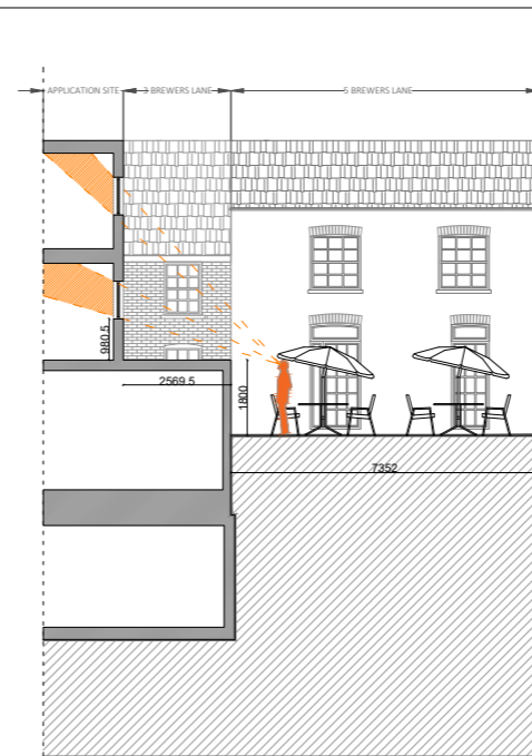
EXISTING SECTION D-D'
