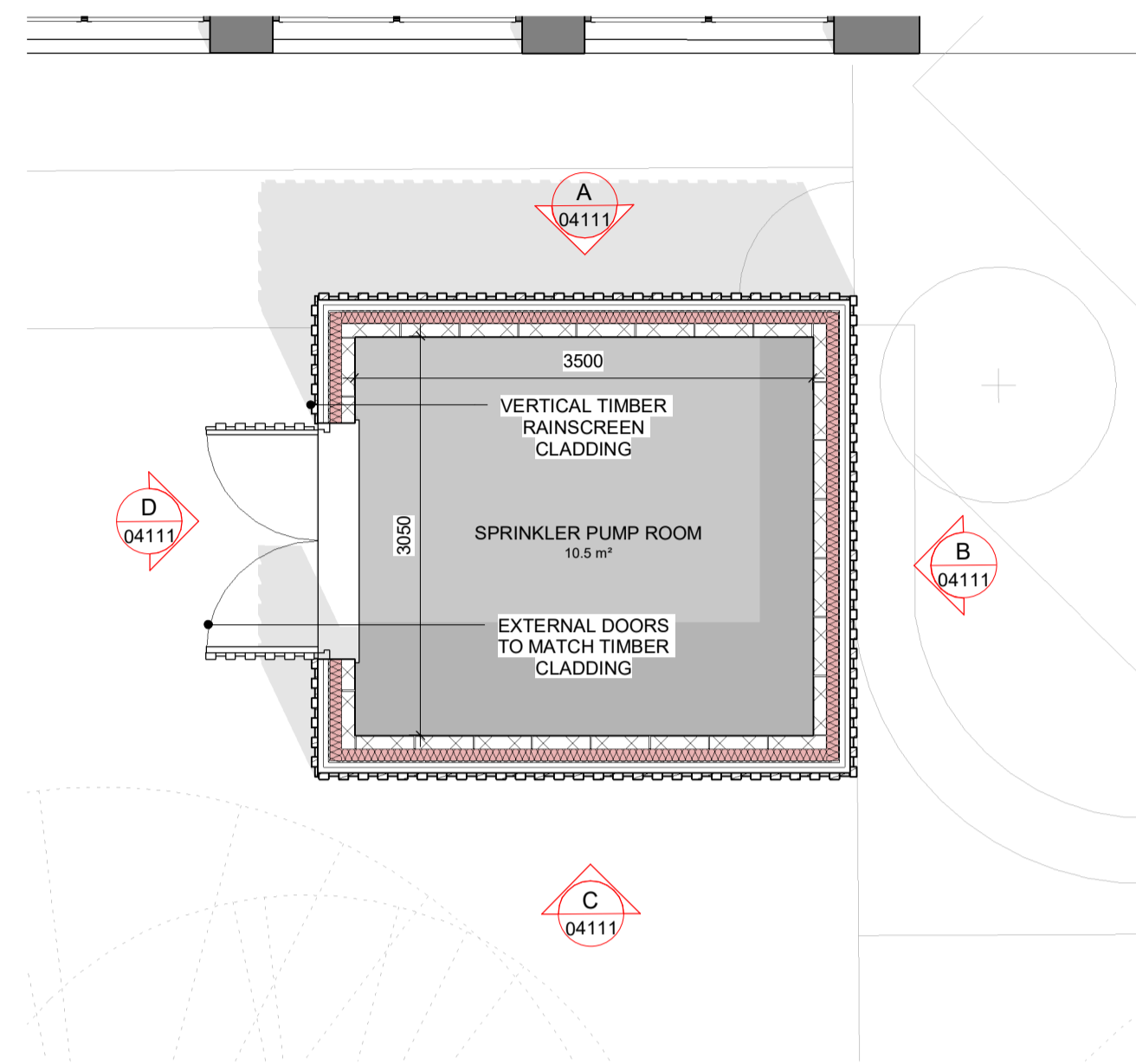
1 SPRINKLER TANK PUMP ROOM - GROUND FLOOR PLAN 1:50
