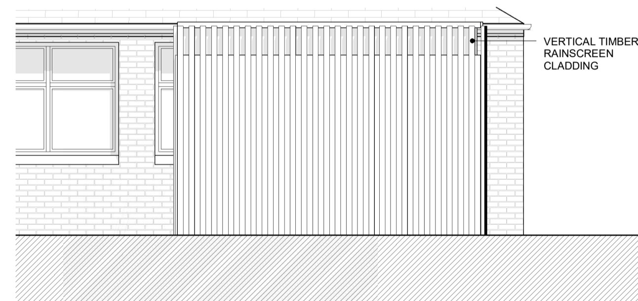
C SPRINKLER TANK PUMP ROOM - SOUTH ELEVATION 1:50
