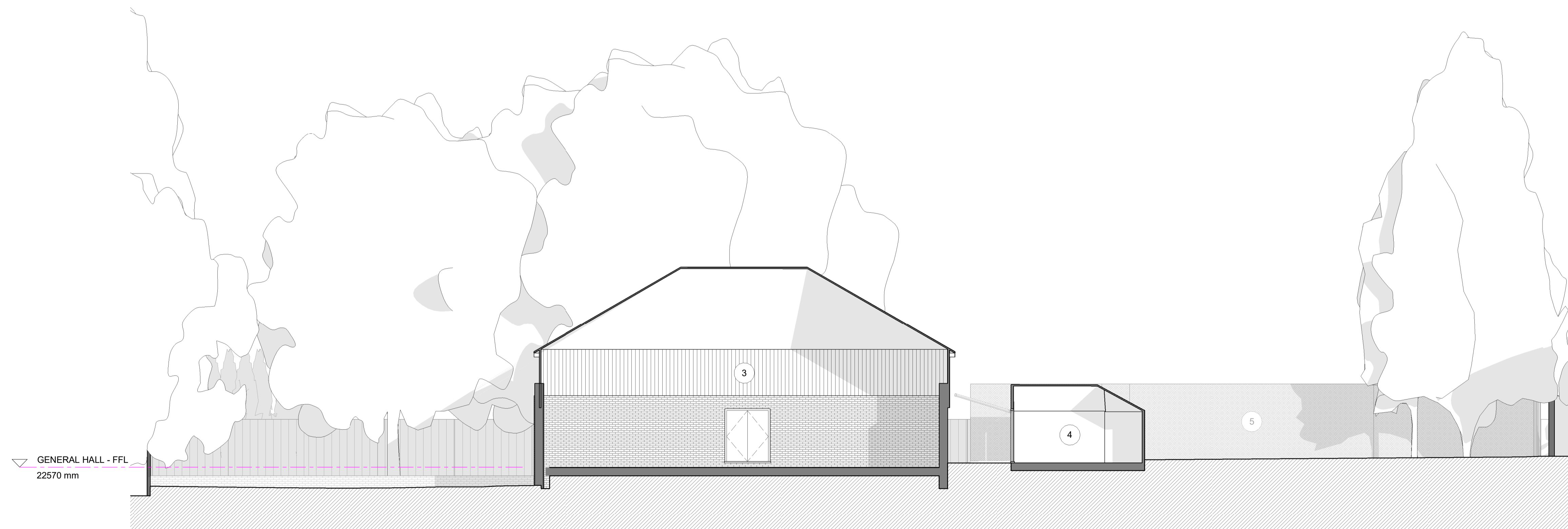
2 EXISTING - SECTION - GENERAL HALL 1:100
