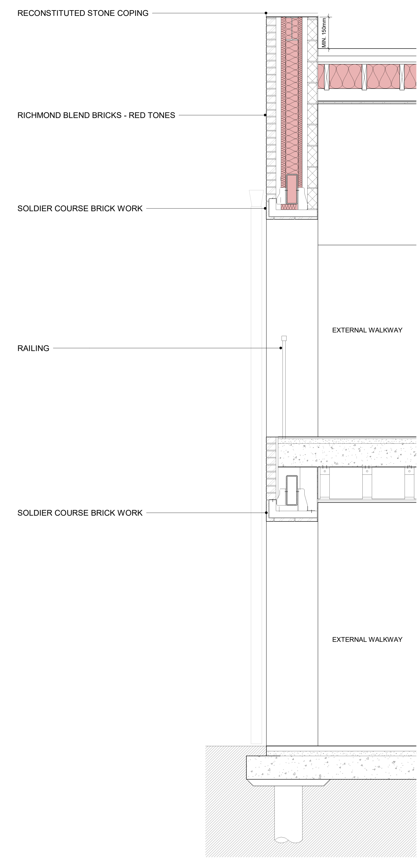
3 PLANNING - SECTION - FACADE DETAIL - BUFF BRICK 1:20
