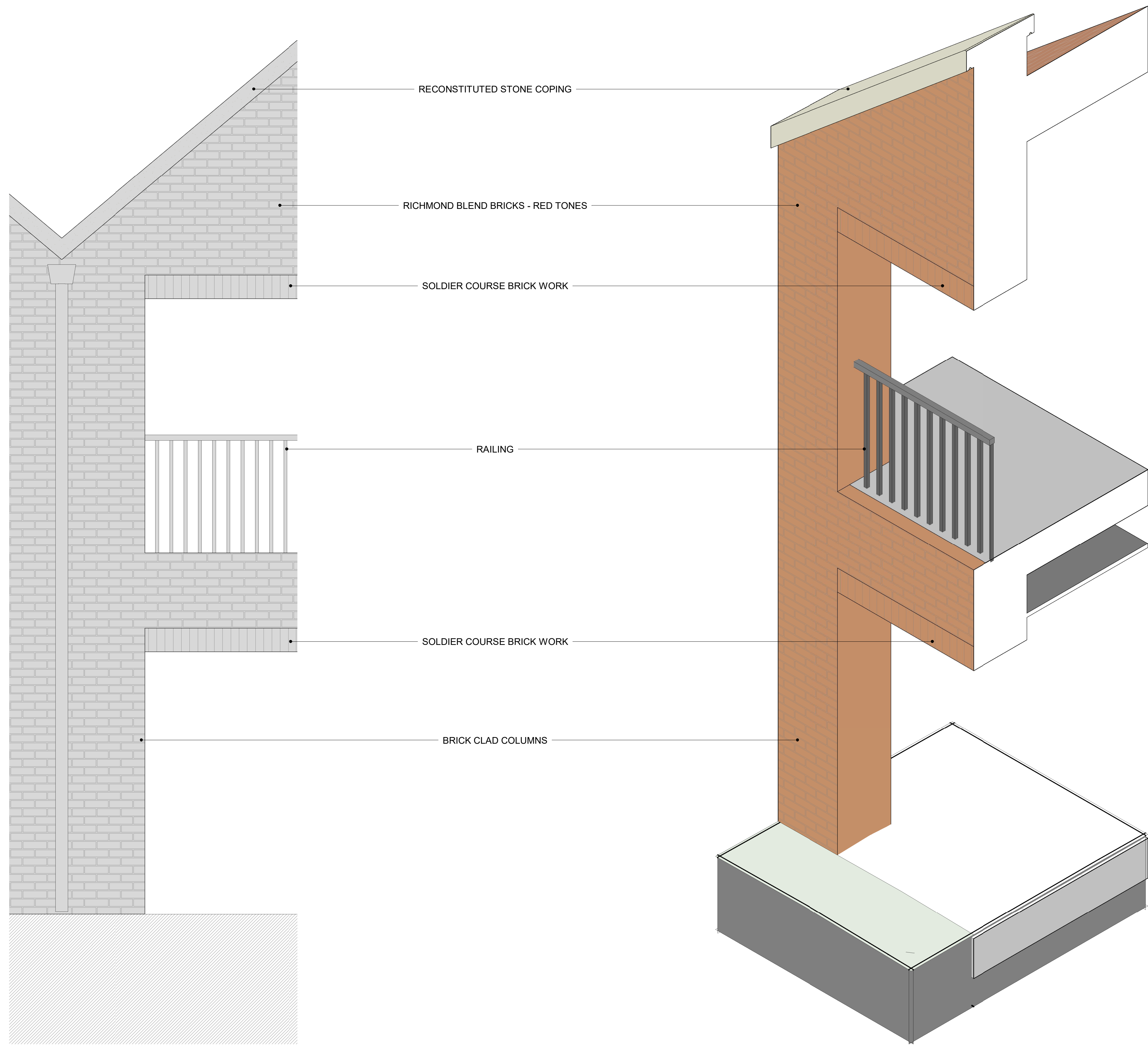
1 PLANNING - ELEVATION - FACADE DETAIL - BUFF BRICK 1:20
