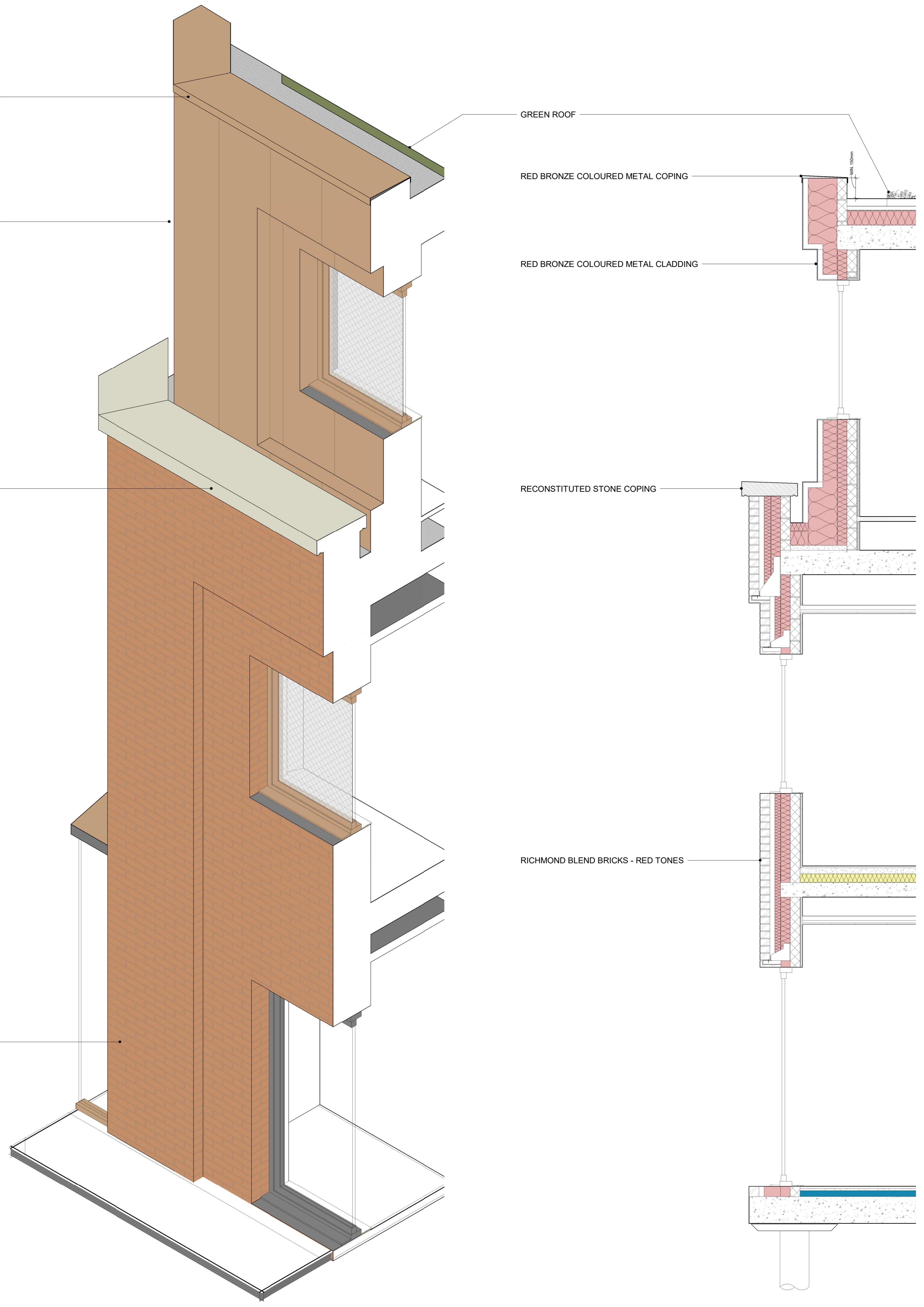
2 3D - PROPOSED FACADE - RED BRICK
