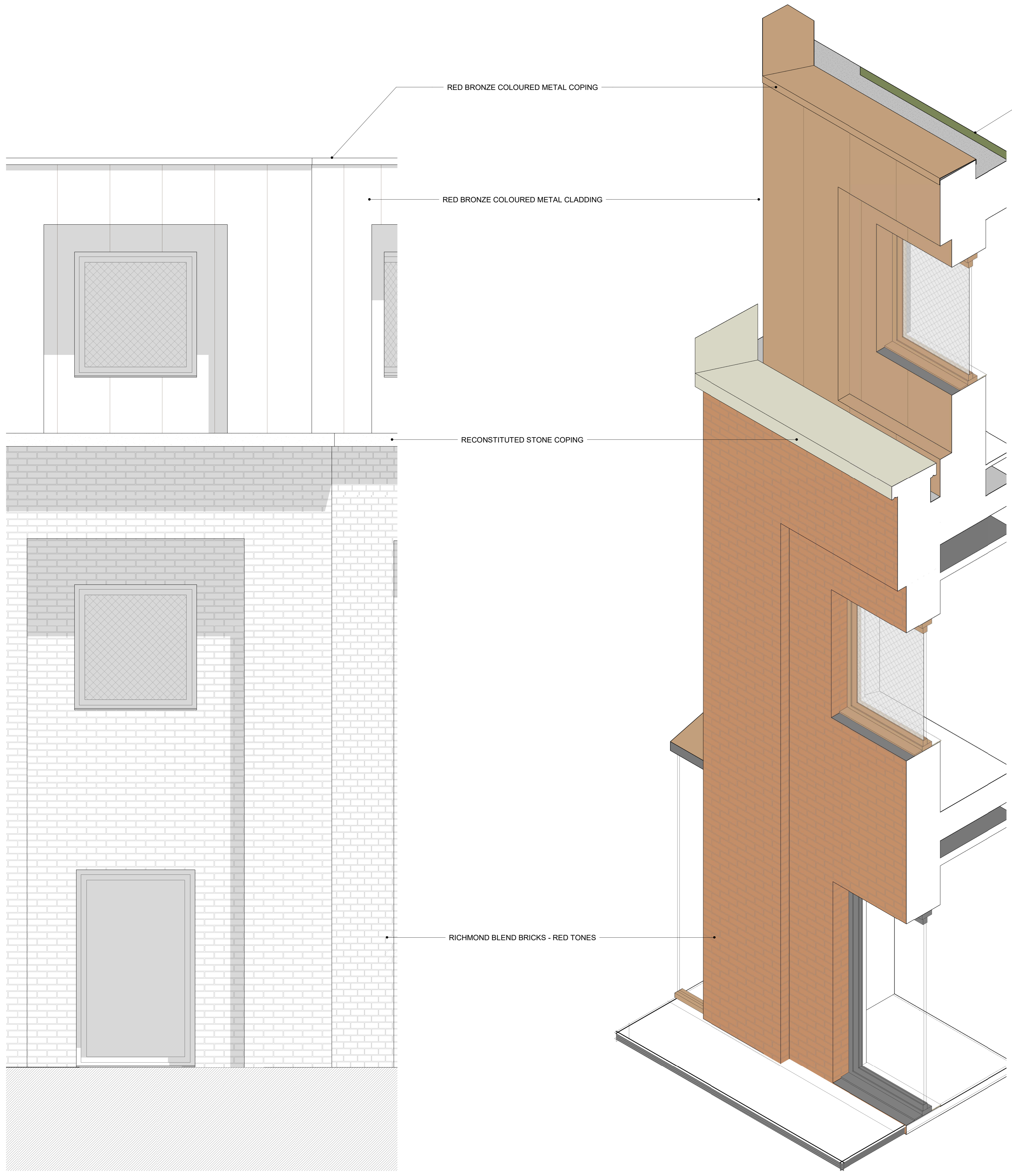
1 PLANNING - ELEVATION - FACADE DETAIL - RED BRICK 1:20
