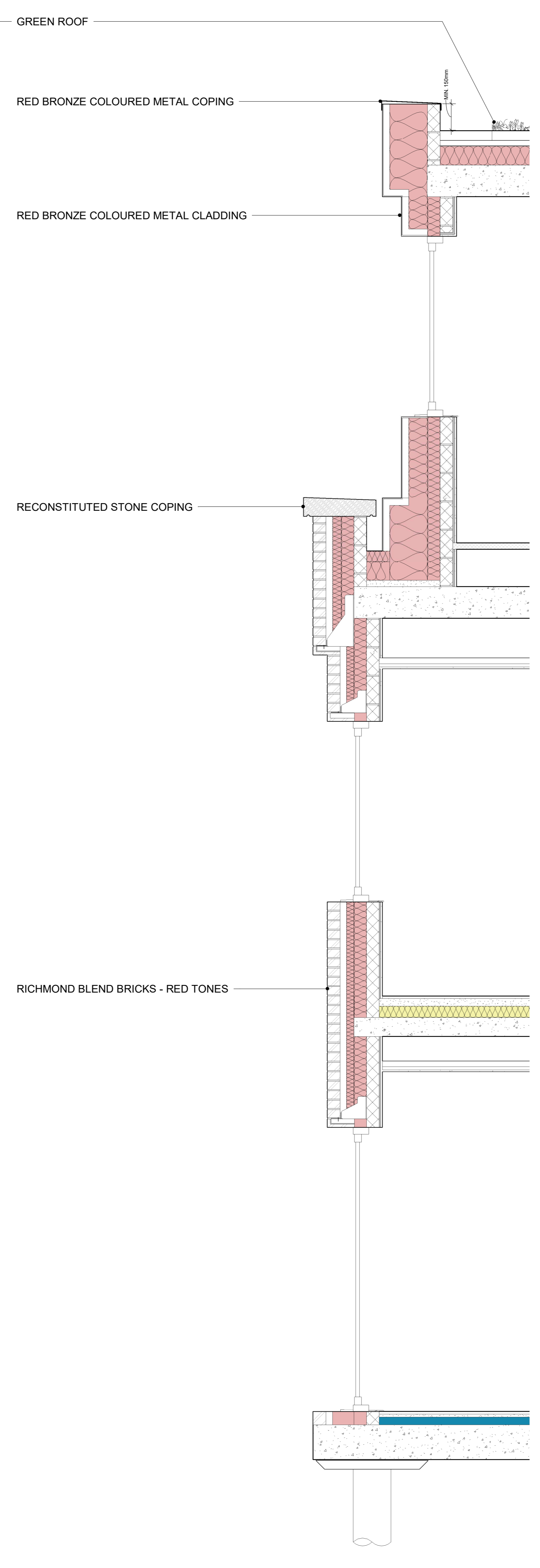
3 Section 45 1:20
