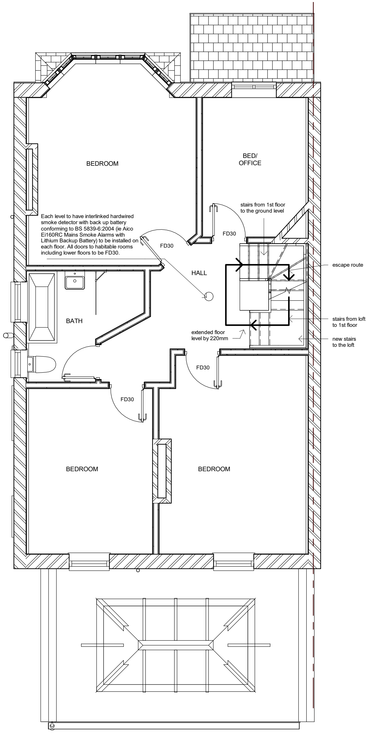
1 PROPOSED FIRST FLOOR PLAN 1 : 50
