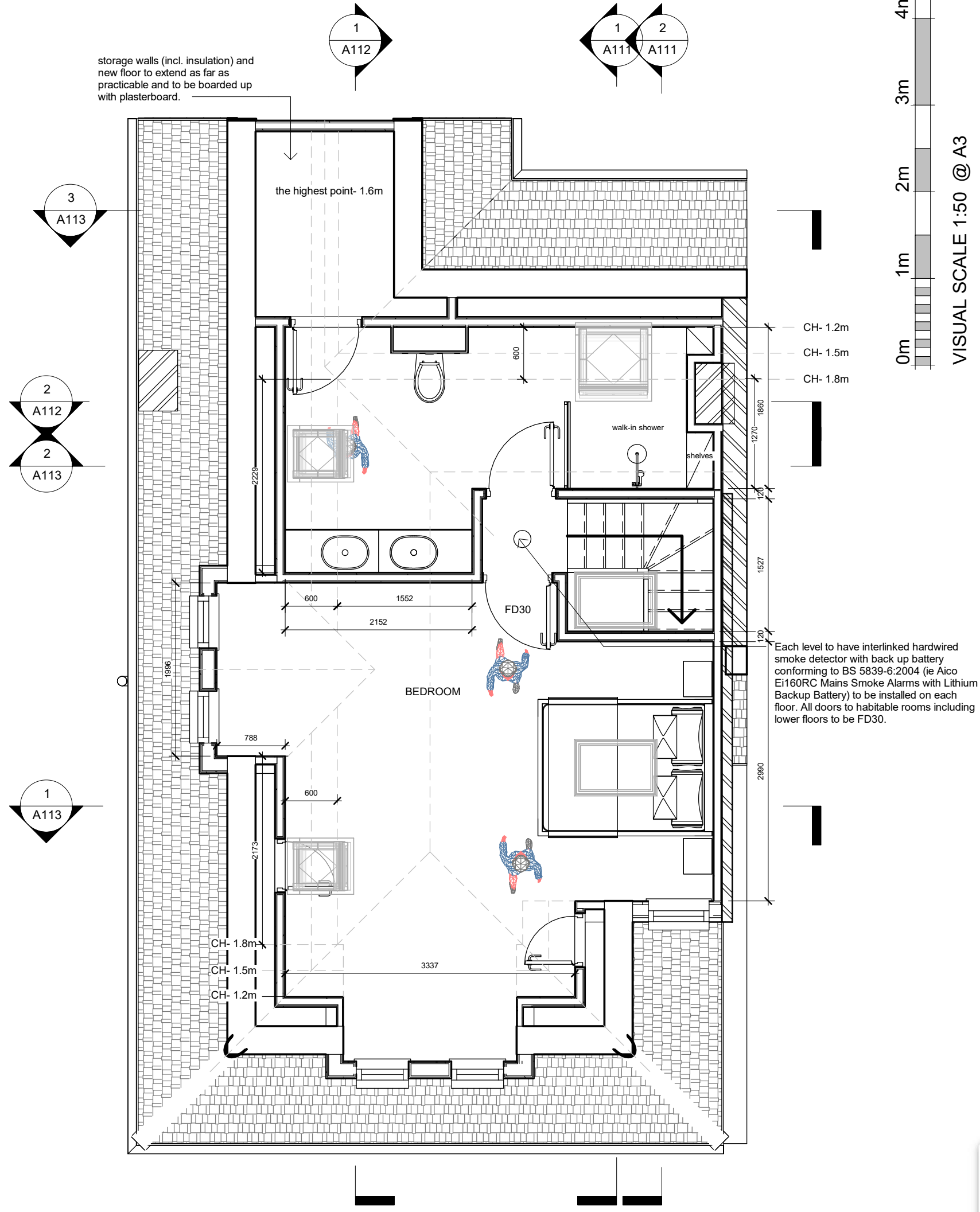
1 PROPOSED LOFT PLAN 1:50
