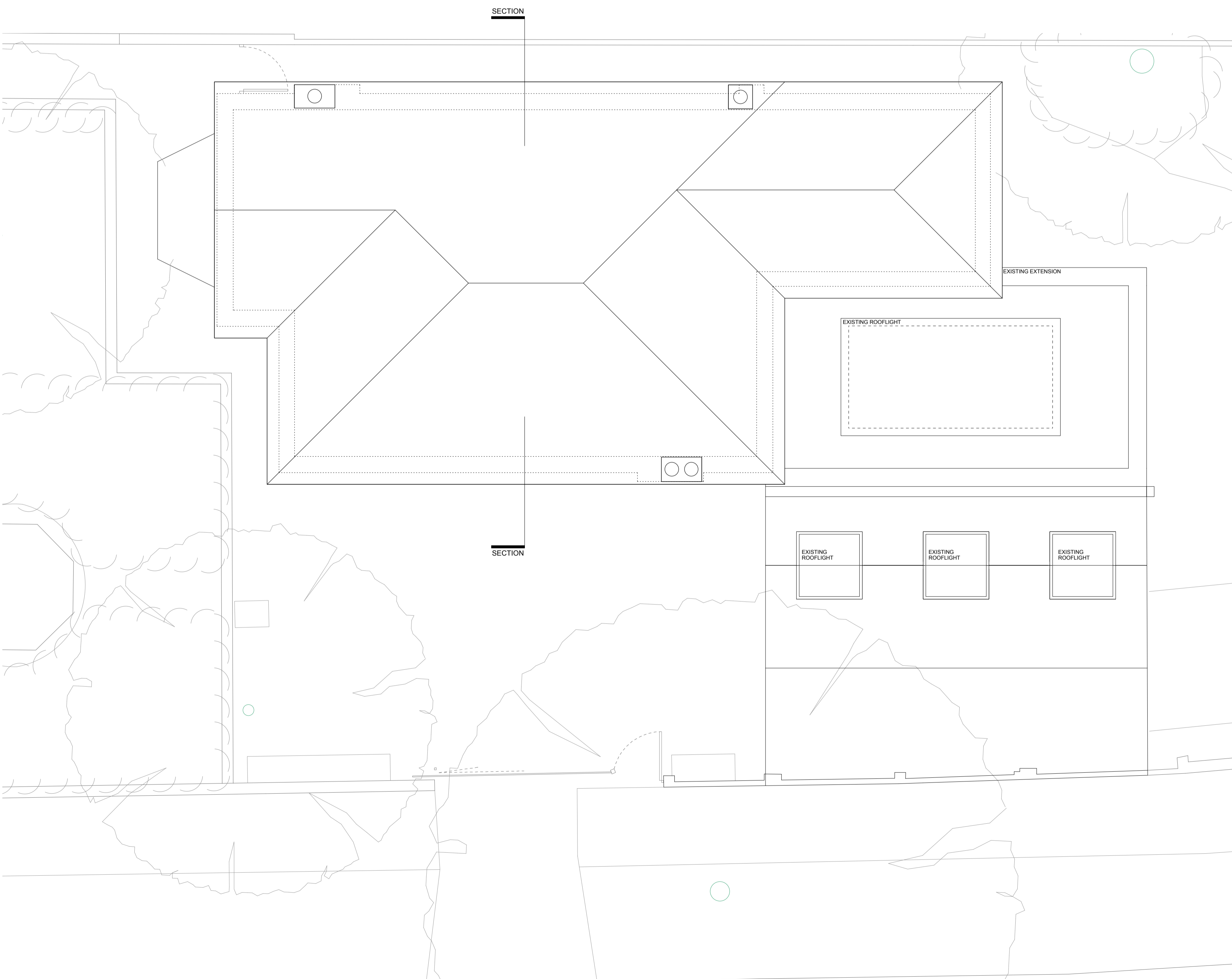
ROOF PLAN
