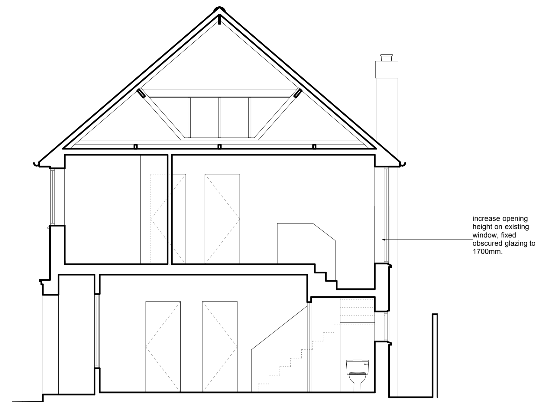
SECTION
