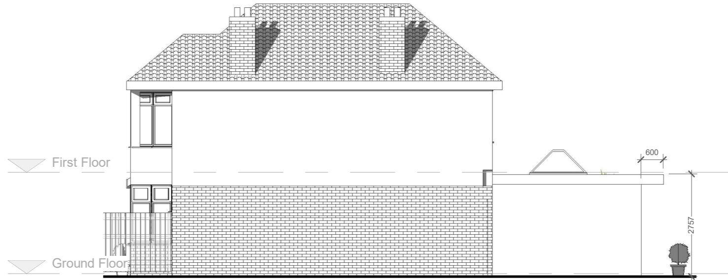
Proposed Right Side Elevation 1 : 100
