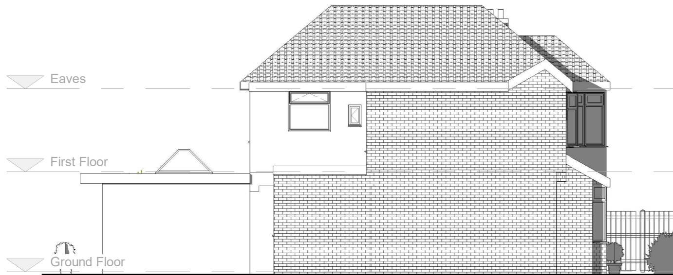
Proposed Left Side Elevation 1 : 100
