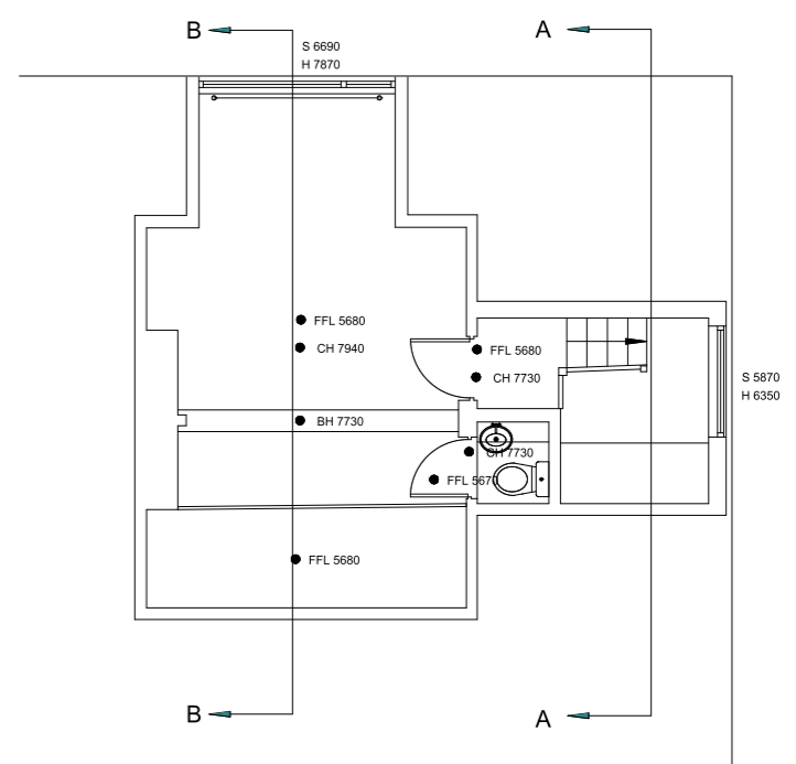
Attic
