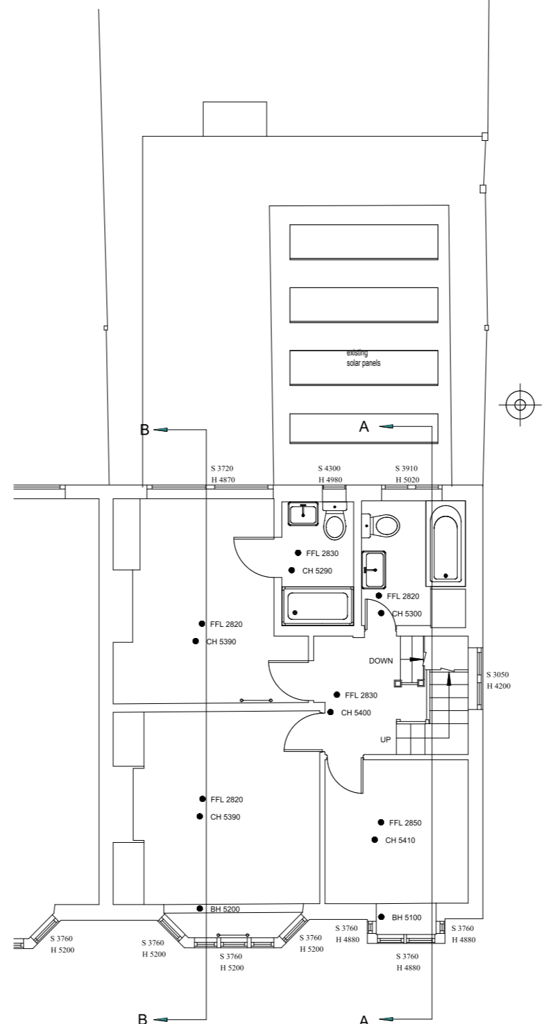
First Floor
