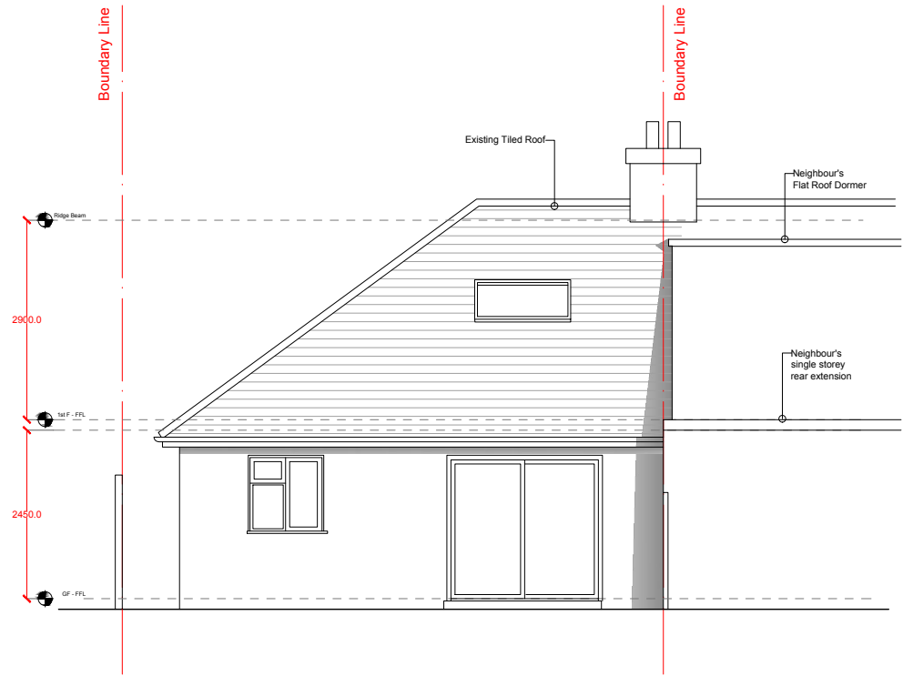
Existing Rear Elevation (B)
