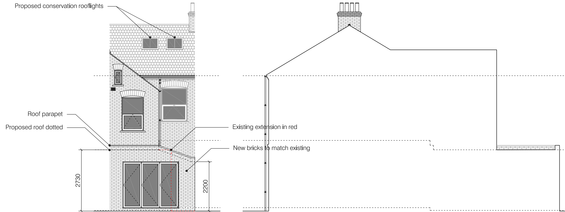
03 Proposed Rear Elevation
