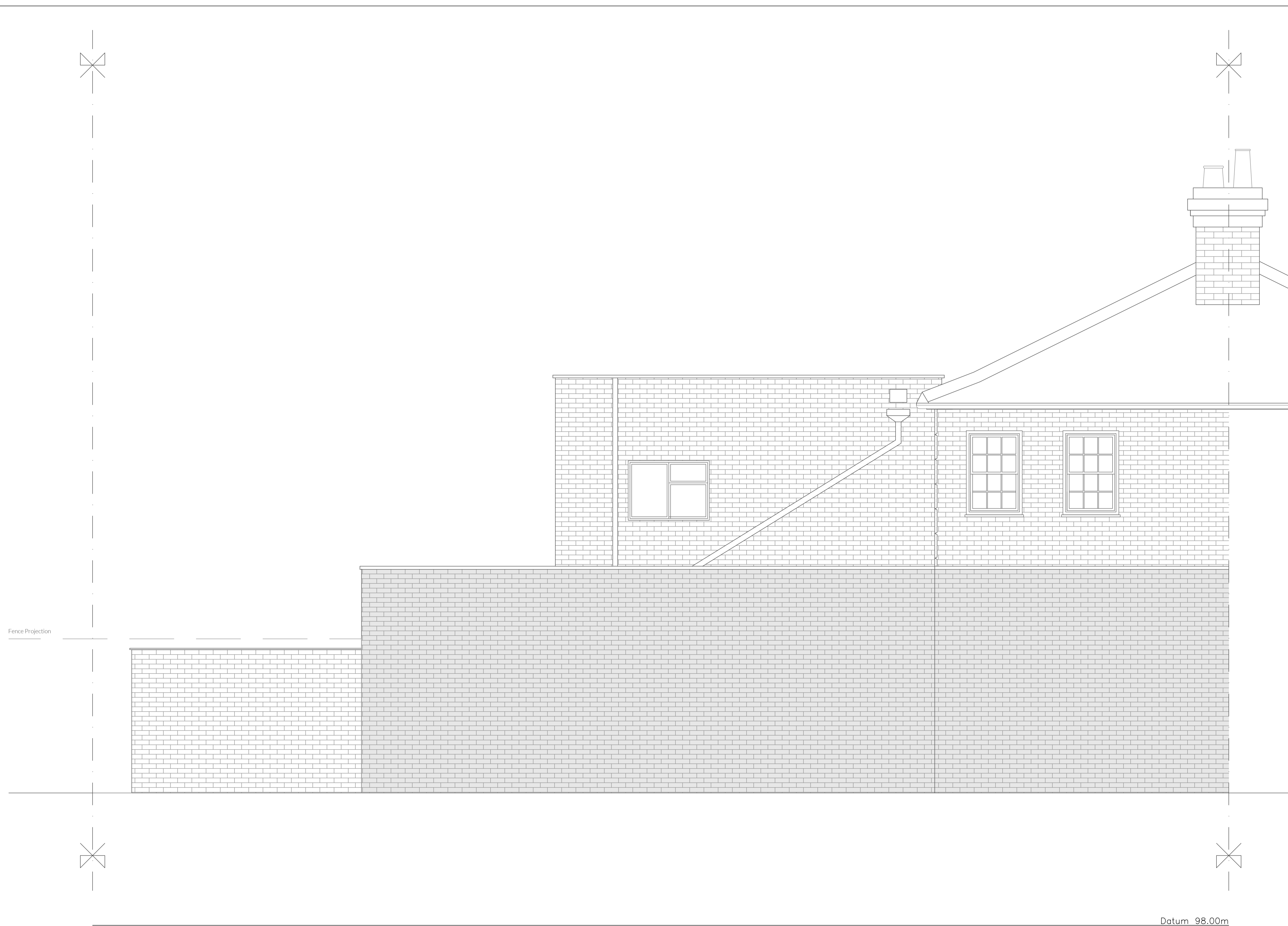
REAR ELEVATION
