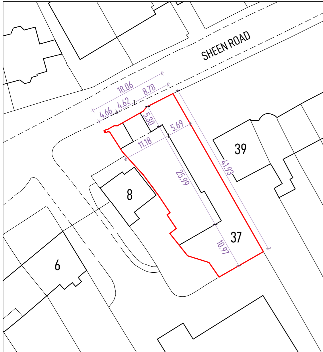
EXISTING SITE PLAN 1:500
