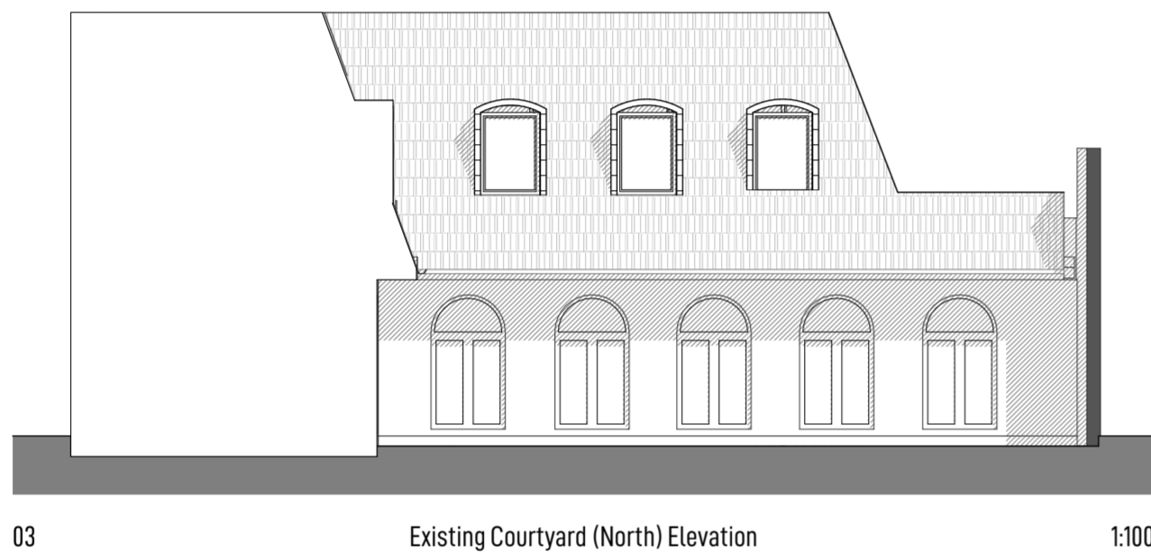
03 Existing Courtyard (North) Elevation 1:100
