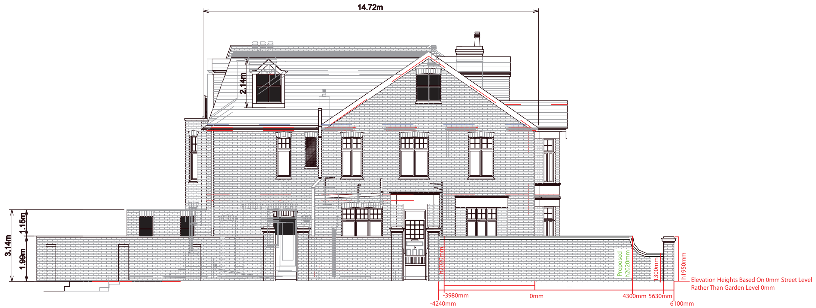
Side Elevation
