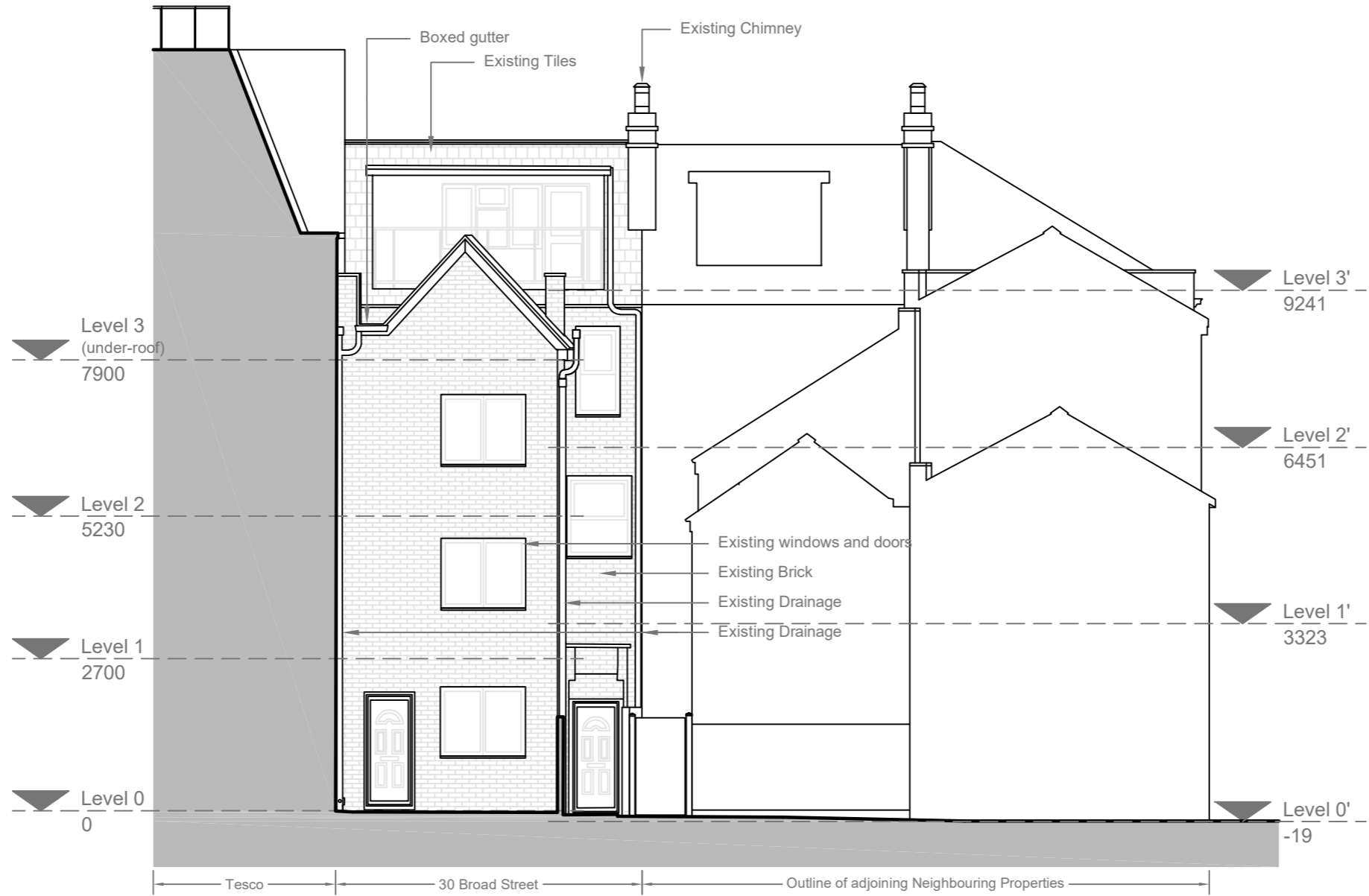
0 1 2 3 4 SOUTH ELEVATION (AS-BUILT)
