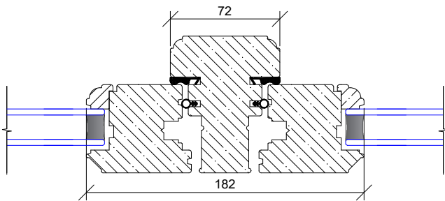
Vertical Mullion
