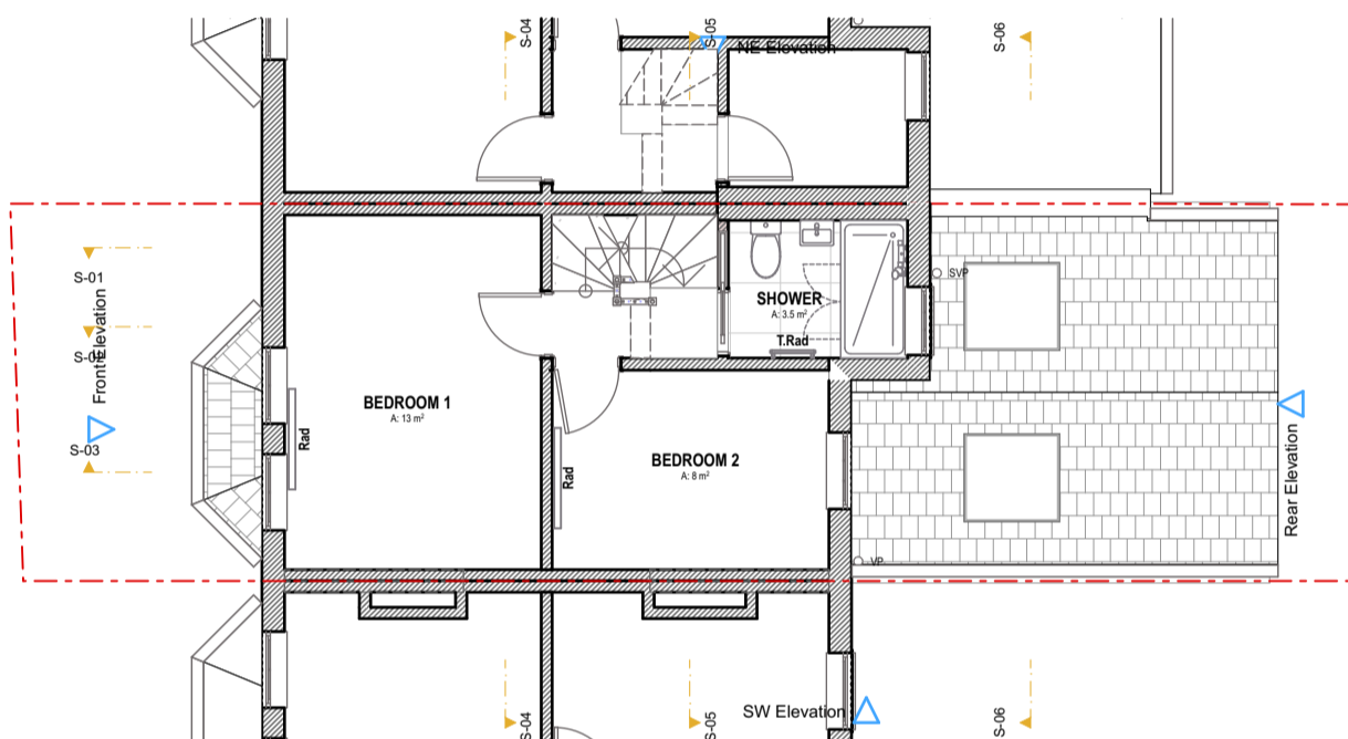
First Floor
