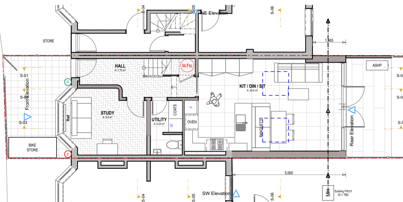
Ground Floor
