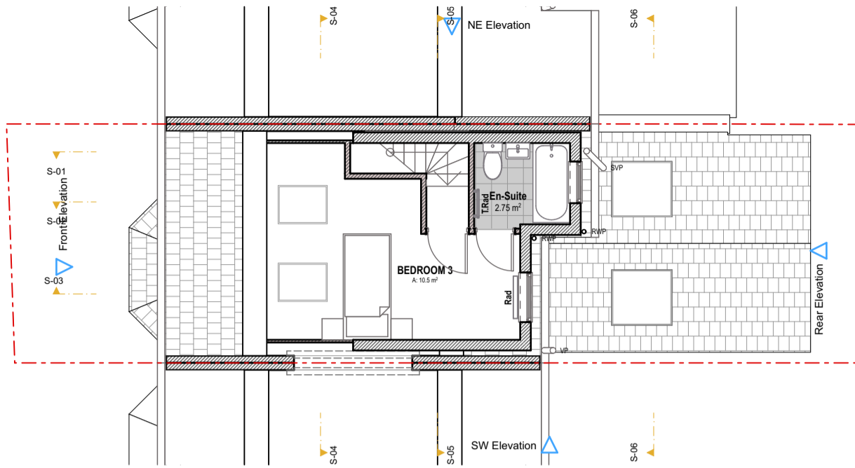
Loft Floor
