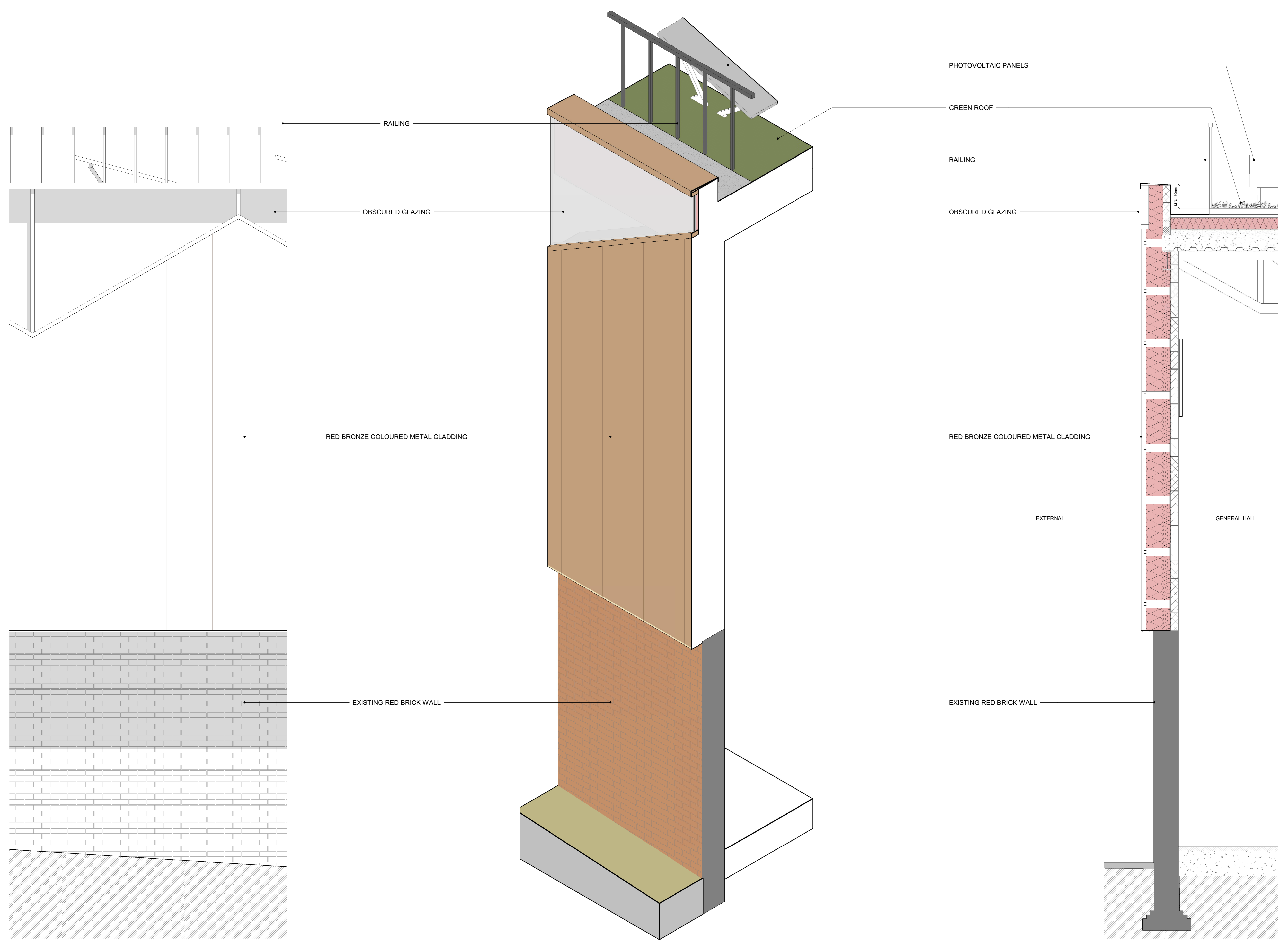
1 PLANNING - ELEVATION - FACADE DETAIL - TIMBER CLADDING 1:20
