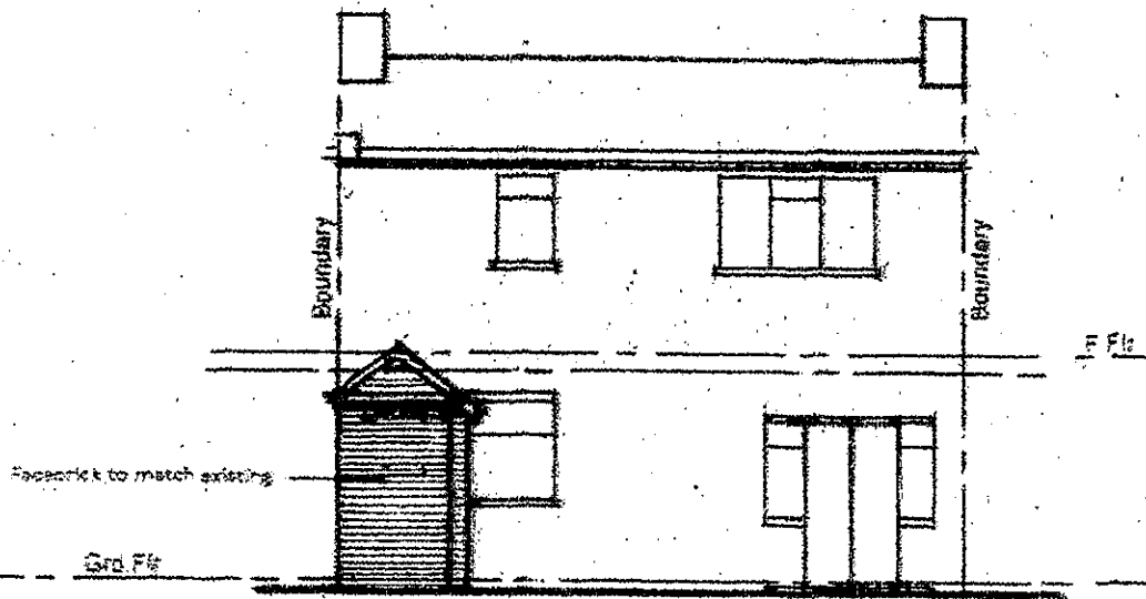
REAR ELEVATION
