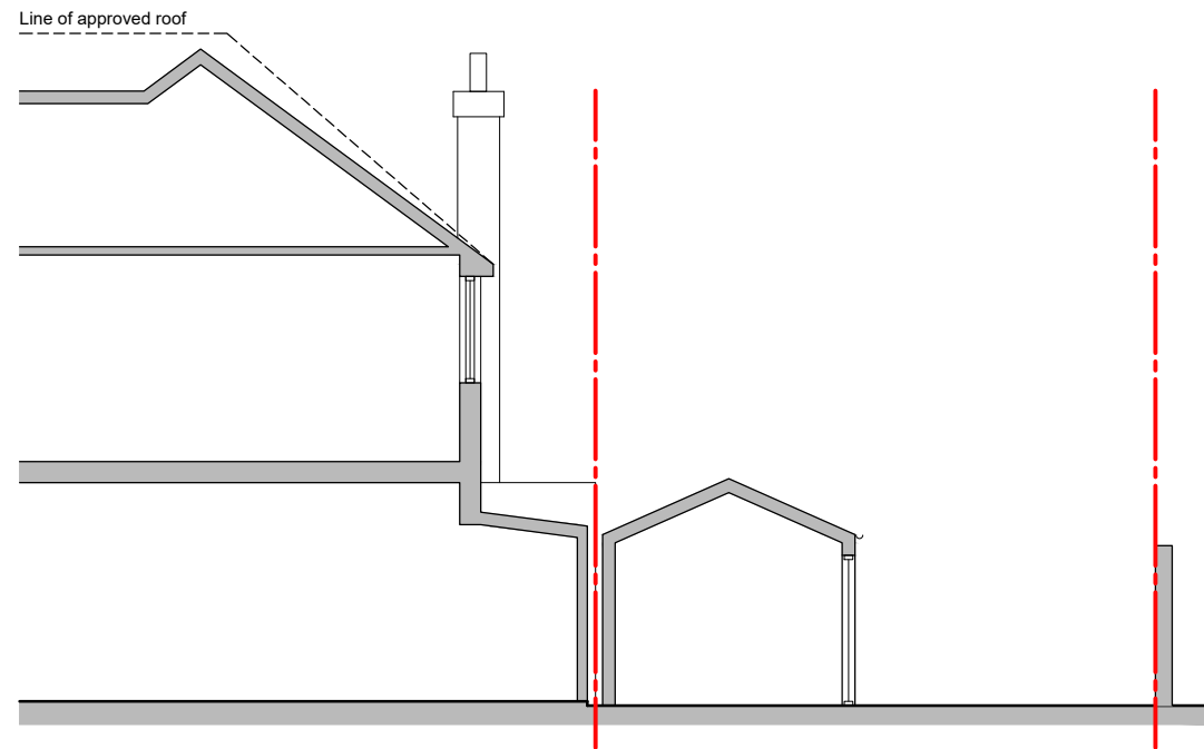
EXISTING SECTION
