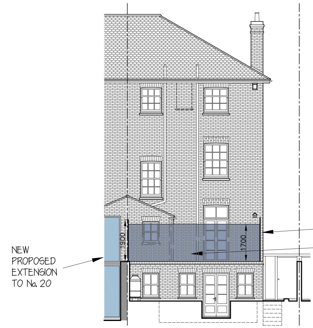
2 - REAR ELEVATION
