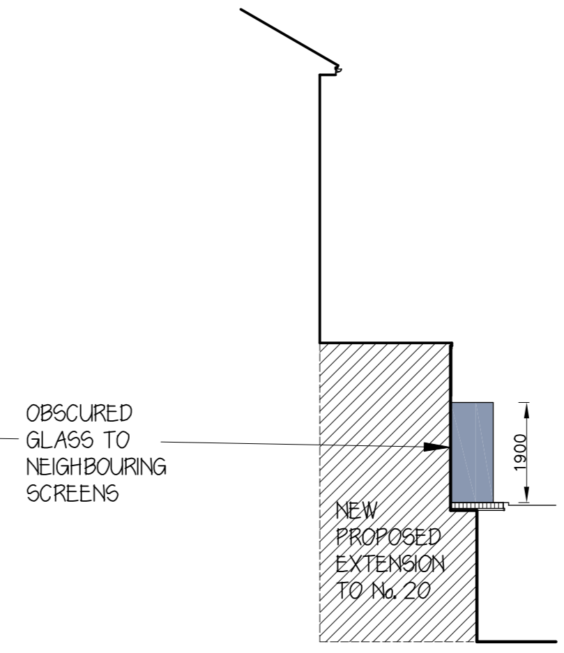
5 - SIDE ELEVATION
