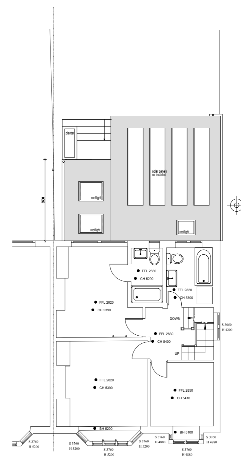
First Floor
