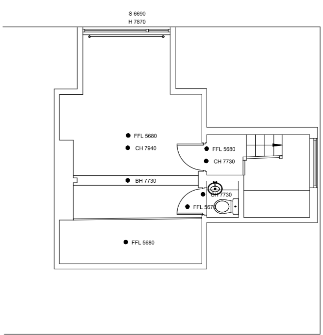
Attic
