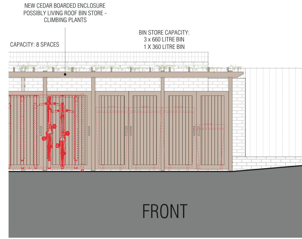
FRONT ELEVATION 1:50
