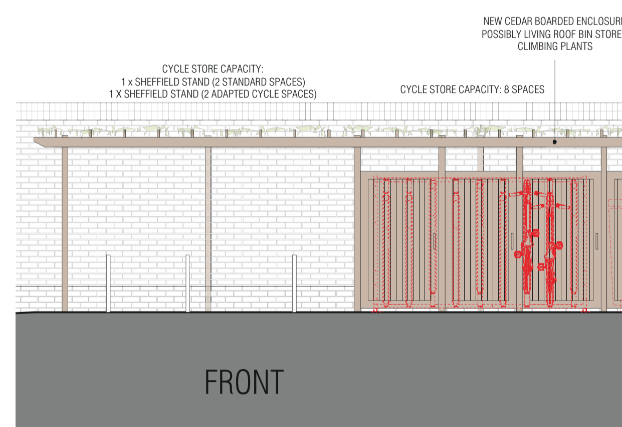
FRONT ELEVATION 1:50
