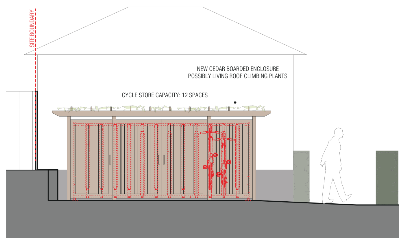
FRONT ELEVATION 1:50
