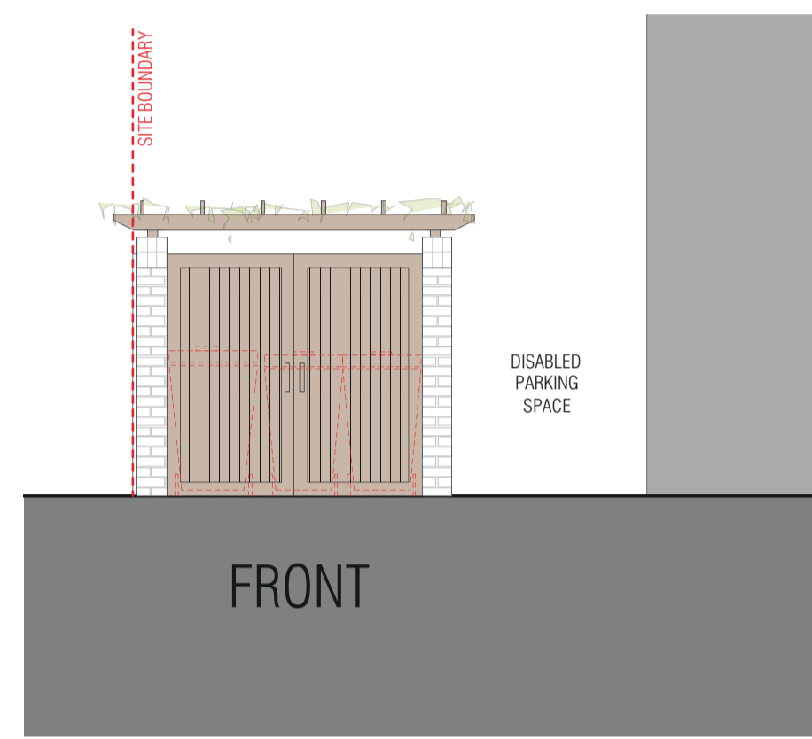
FRONT ELEVATION 1:50
