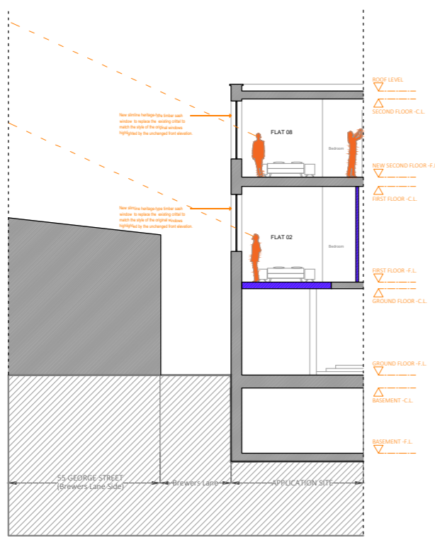
PROPOSED SECTION A-A'
