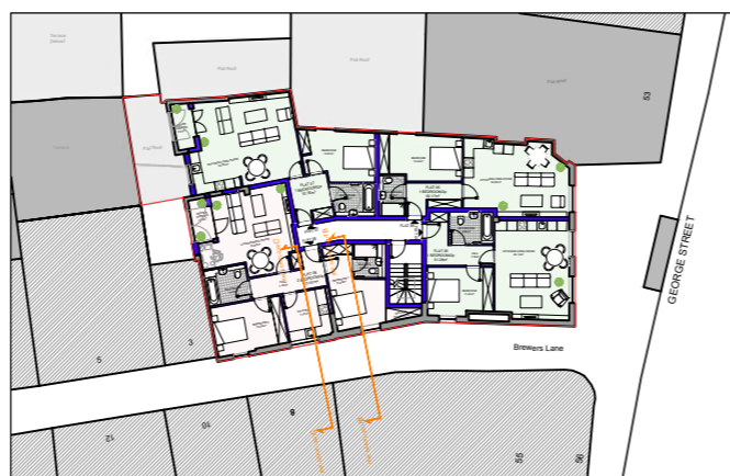
PROPOSED SECOND FLOOR
