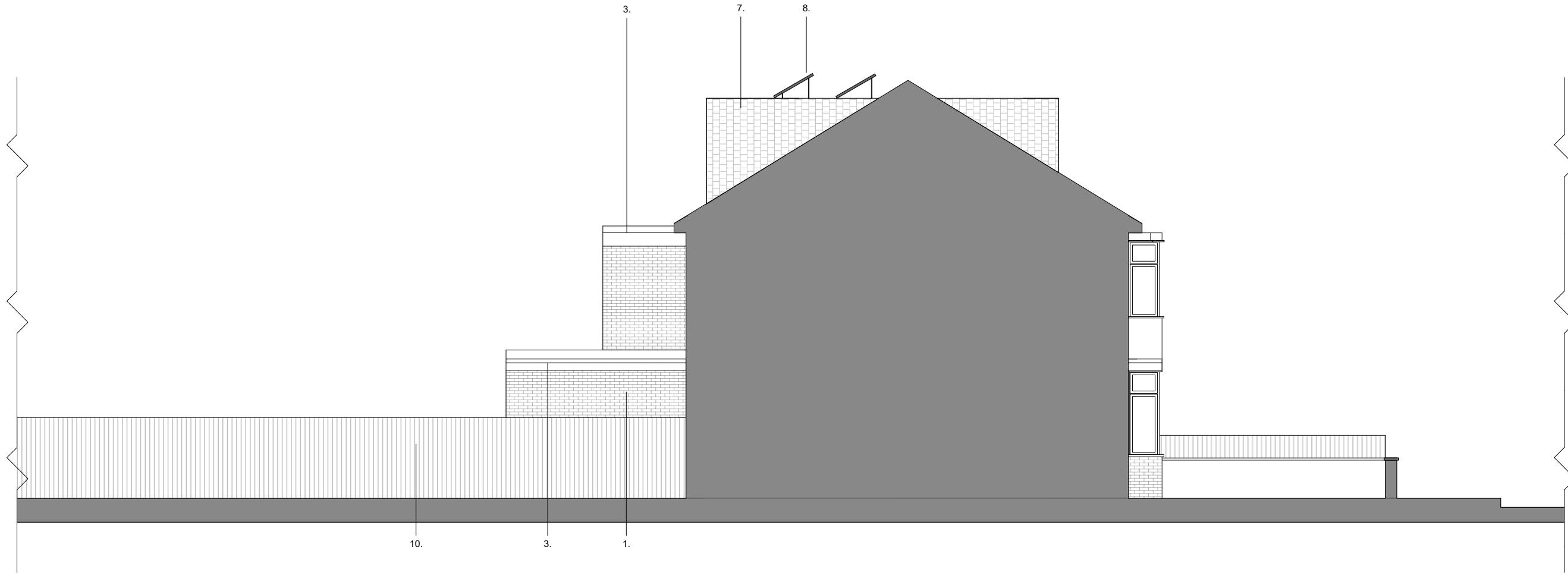
10 Proposed East Elevation Scale: 1:100
