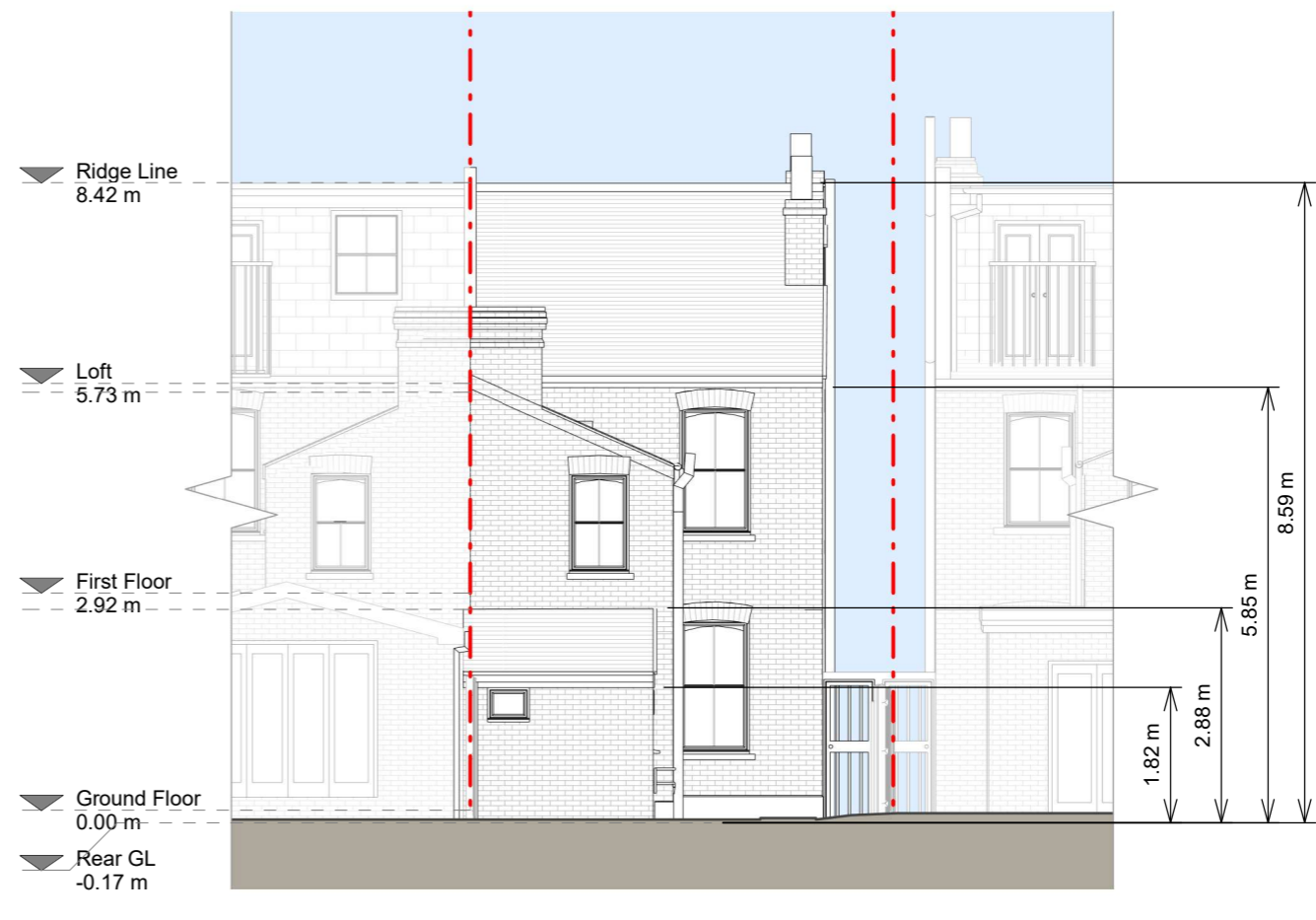
Rear Elevation
