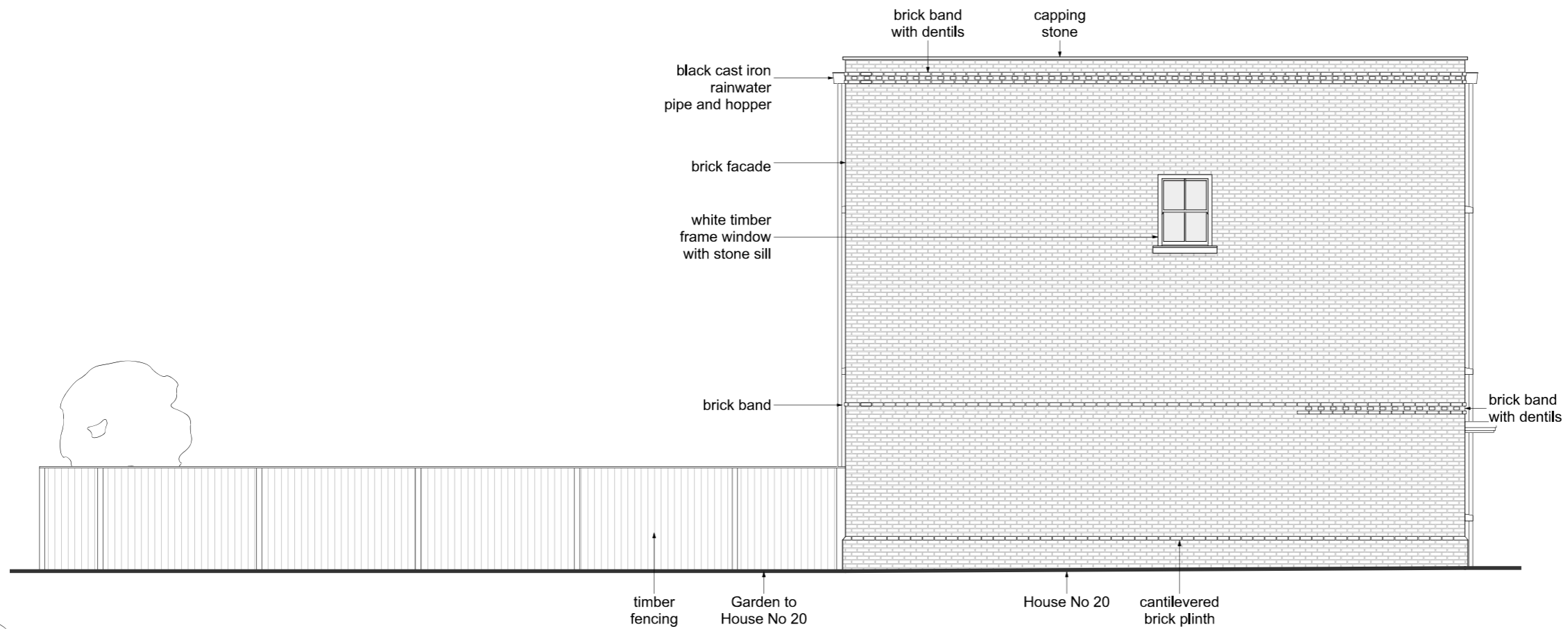
1 005 EXISTING SIDE ELEVATION WEST
