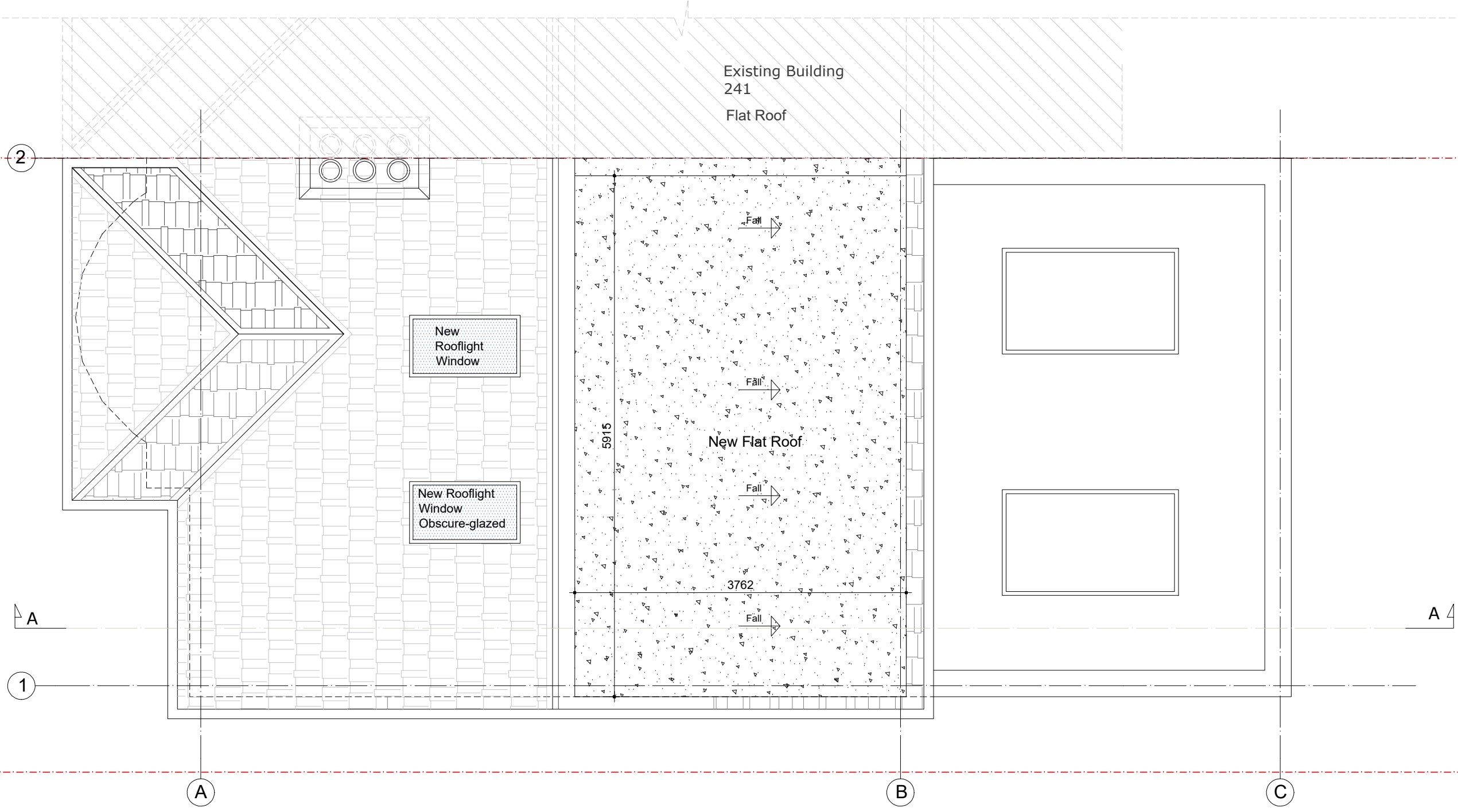
PROPOSED ROOF PLAN P.100 SCALE 1:50
