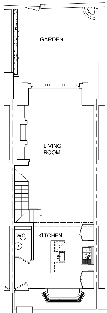
GROUND FLOOR PLAN scale 1:125
