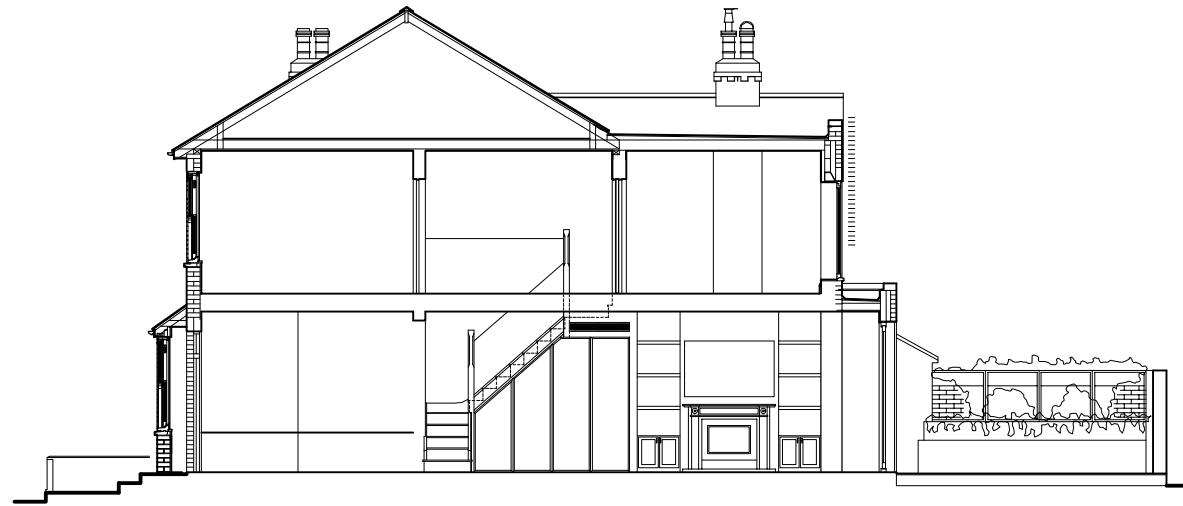
GENERAL SECTION scale 1:125
