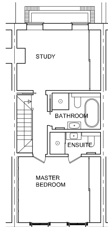
FIRST FLOOR PLAN scale 1:125
