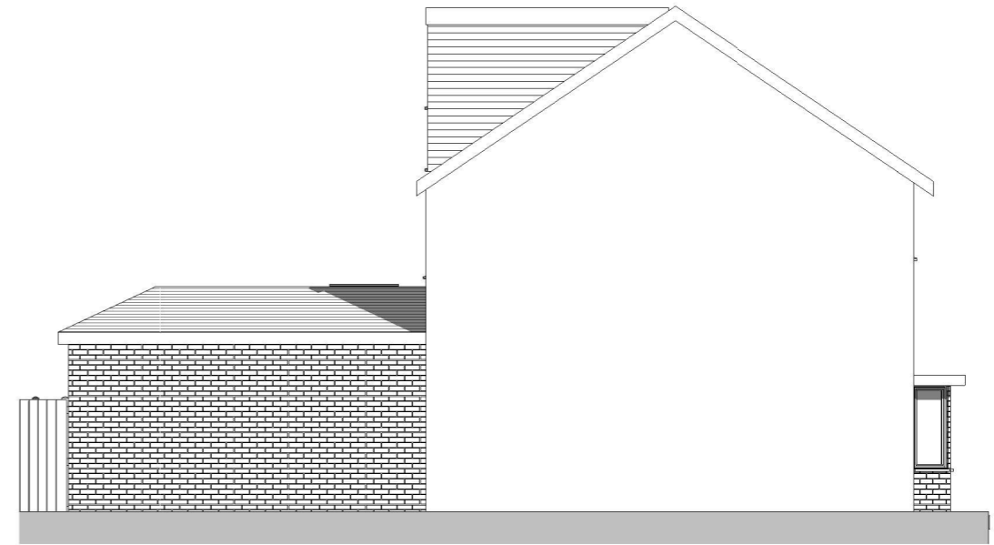
Proposed Side 1 Elevation 1 : 100
