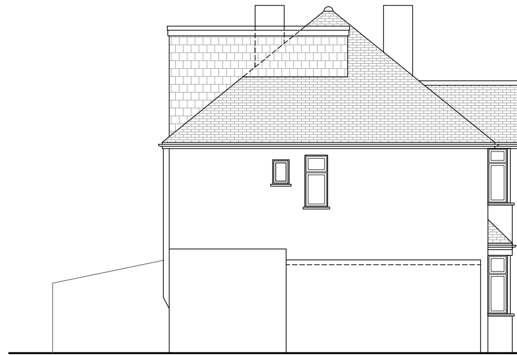
Existing RHS Elevation Scale 1/100@A3
