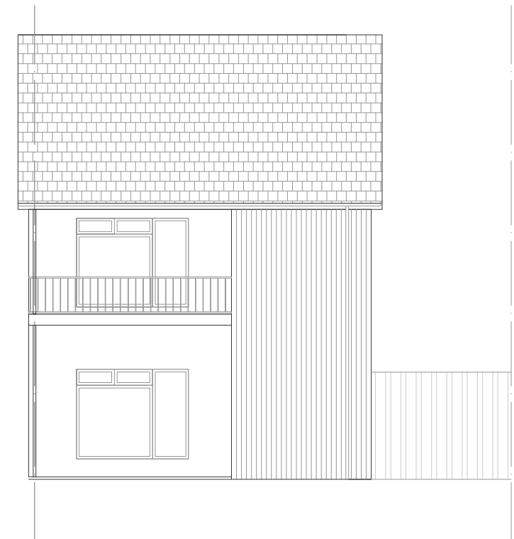
FRONT ELEVATION E: 1/100
