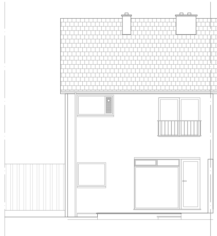
REAR ELEVATION E: 1/100
