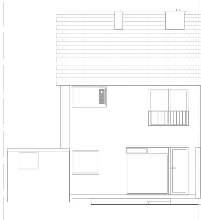
REAR ELEVATION showing ex. garage E: 1/100
