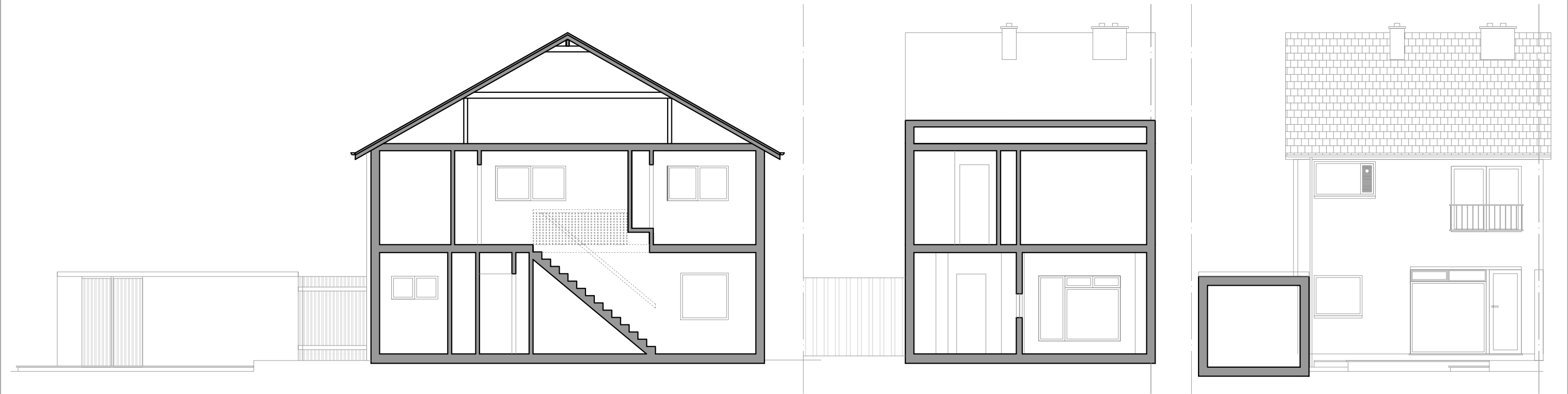
SECTION AA E: 1/100
