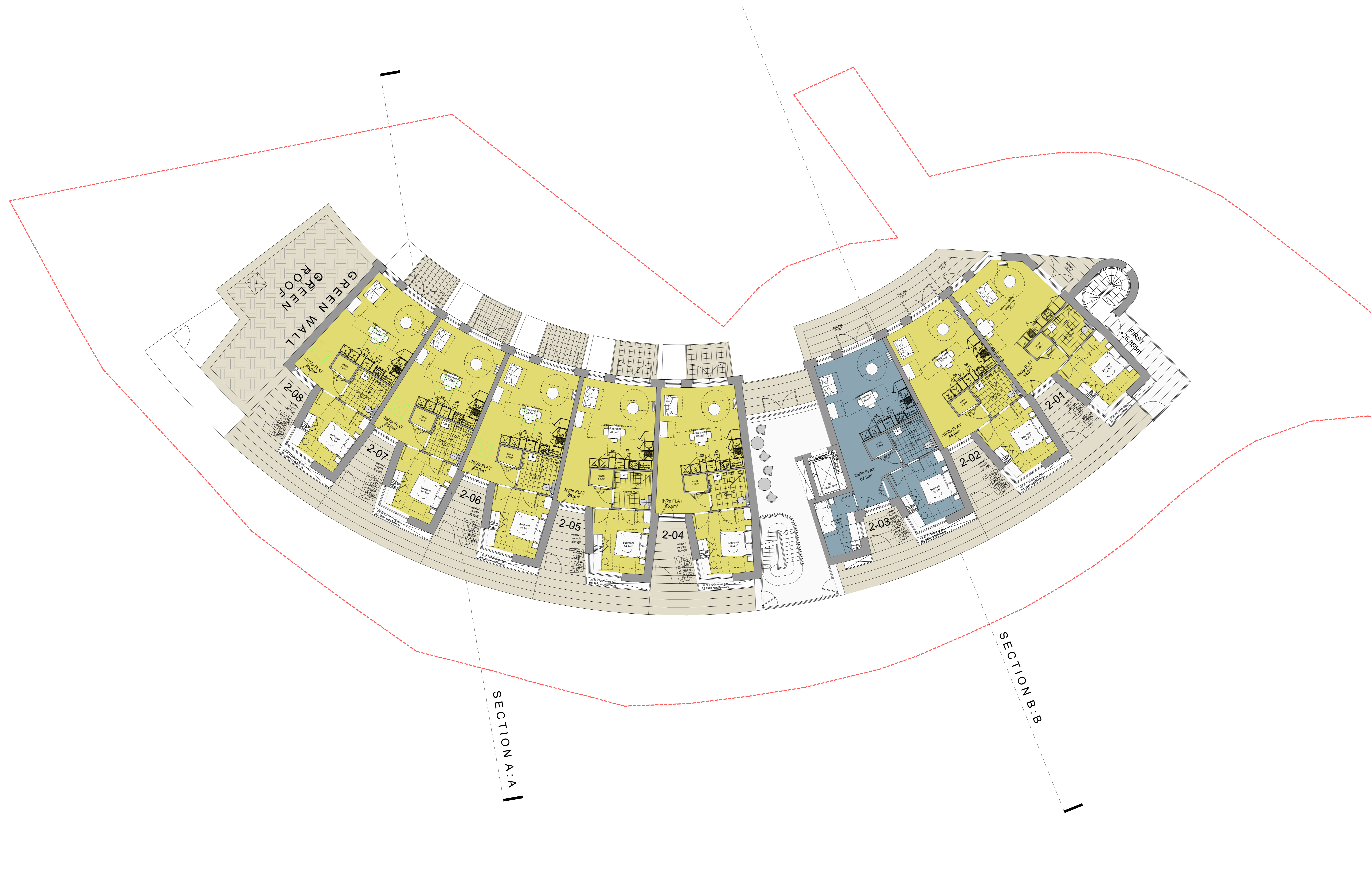
FIRST FLOOR PLAN scale 1:100@A0
