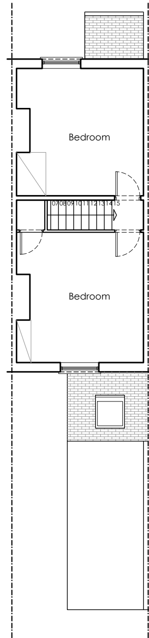
Existing First Floor Plan Scale 1/100@A3
