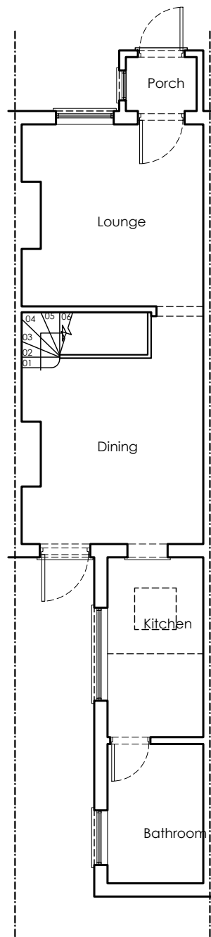
Existing Ground Floor Plan Scale 1/100@A3
