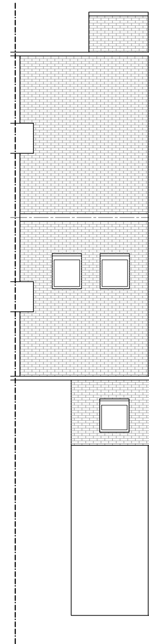
Existing Roof Plan Scale 1/100@A3
