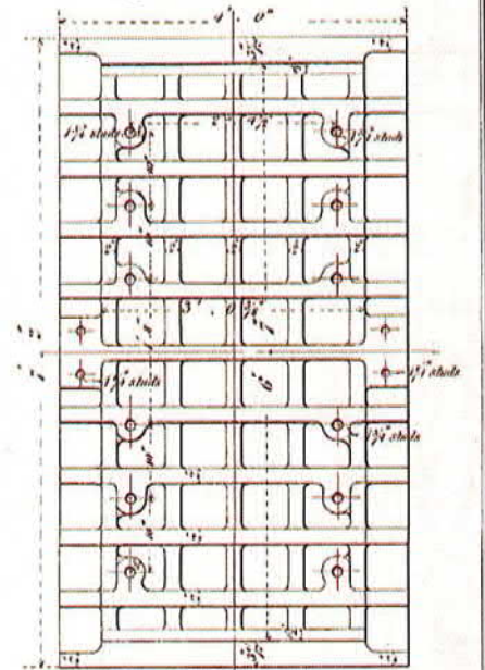
Plan of Upper Roller Plate
