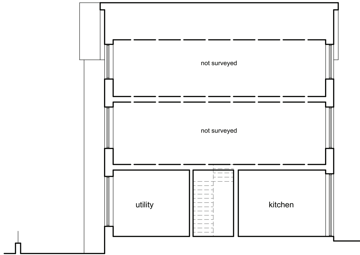
SECTION A-A as existing
