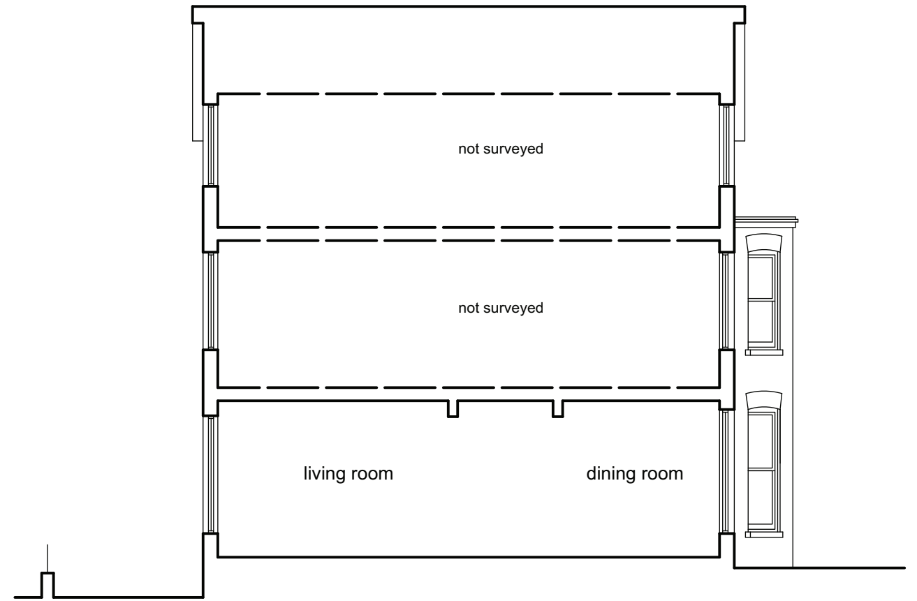
SECTION B-B as existing
